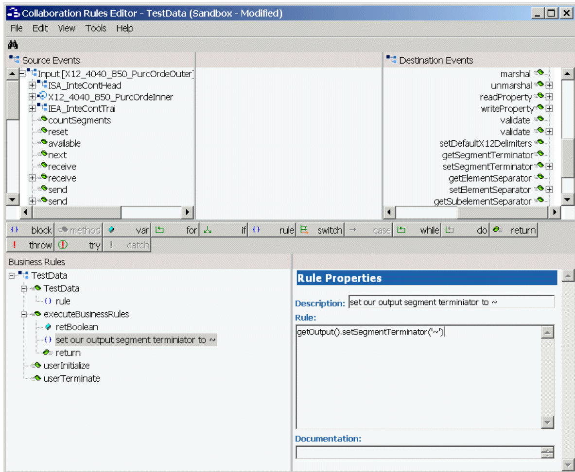
Figure 18 Setting Delimiters in a Collaboration Rules Component
