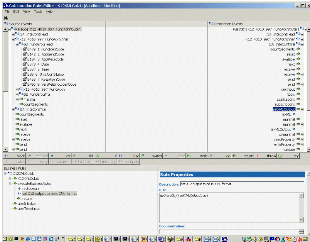
Figure 24 Setting the Output to XML in the X12 Collaboration
