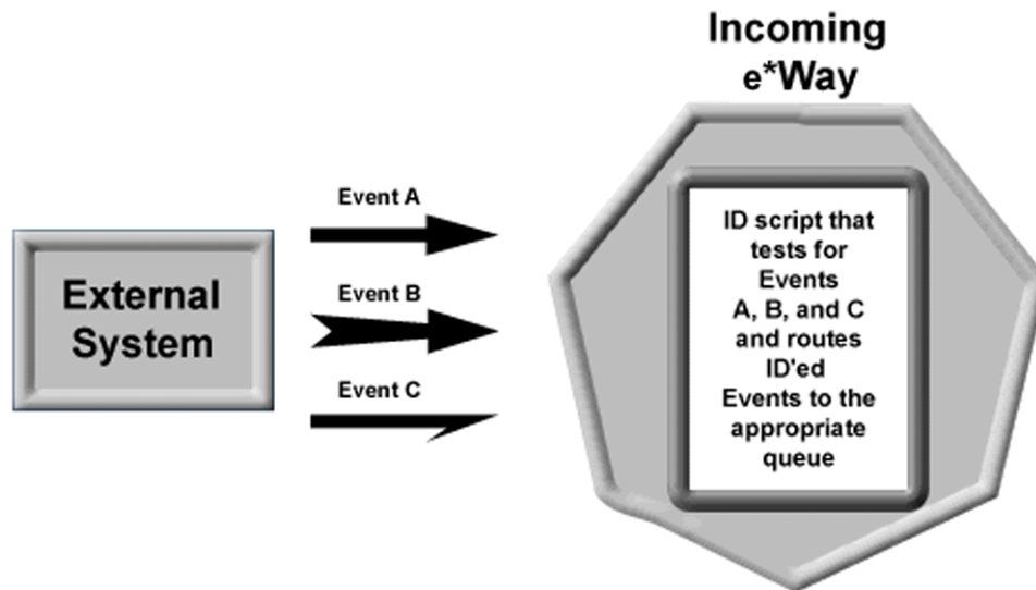
Figure 4 A single Collaboration Rules script for multiple IDs
