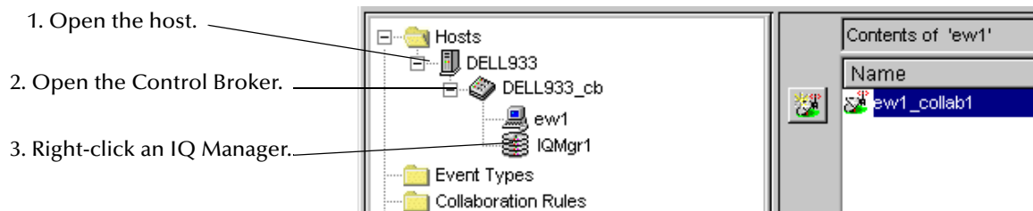
Figure 9 Enterprise Manager with Components Displayed
