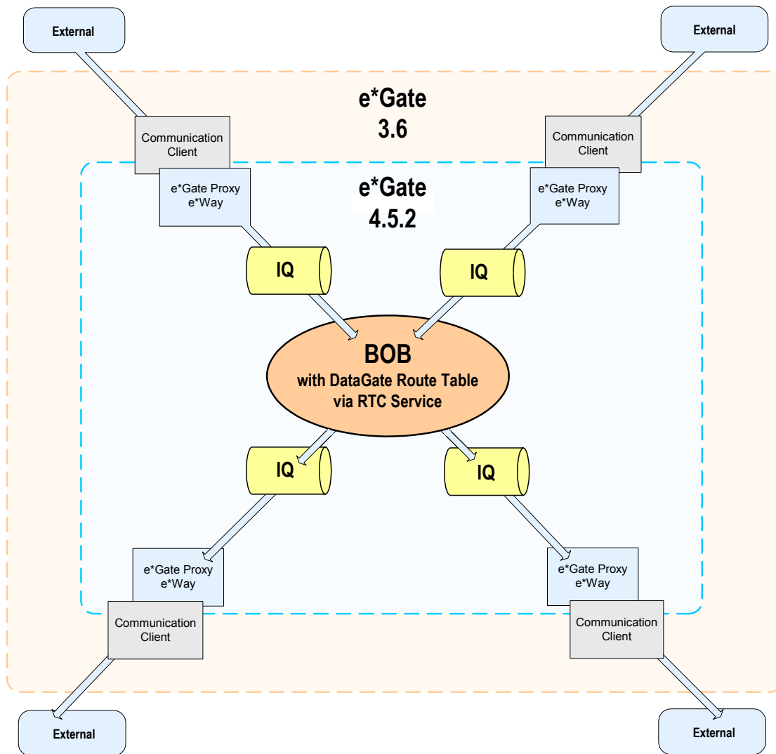
Figure 5 Associates Route with Single BOB in e*Gate 4.5.2
