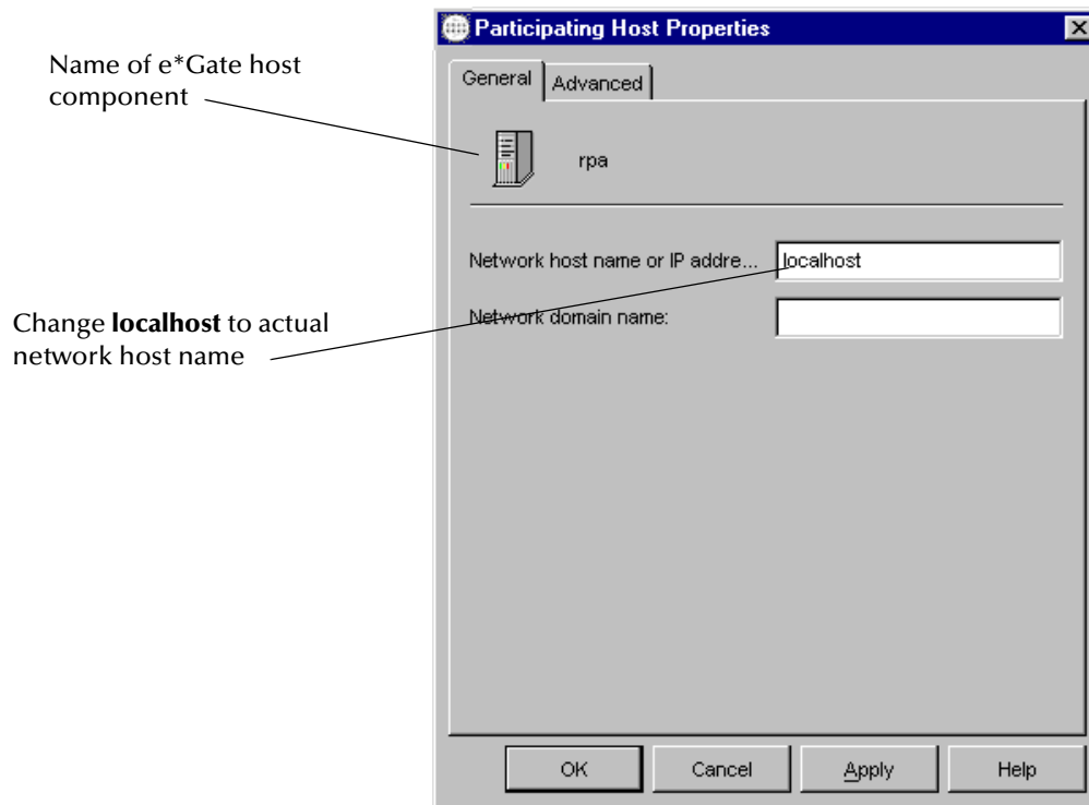
Figure 8 Participating Host Properties Dialog Box
