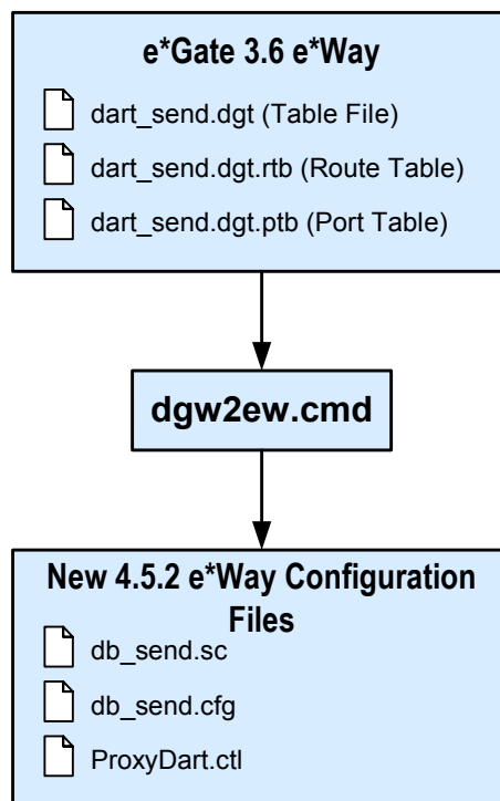
Figure 17 New e*Way Configuration Files
