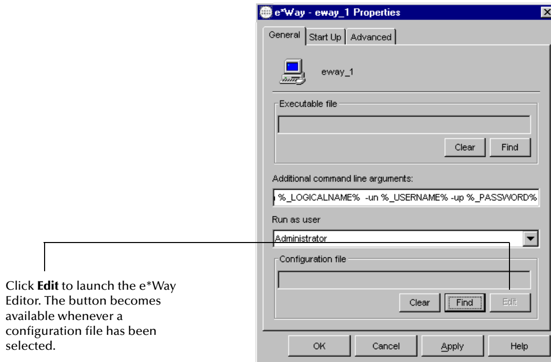
Figure 16 e*Way Properties Dialog Box Showing the Edit Button
