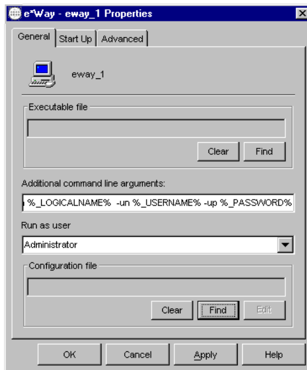
Figure 15 Finding the e*Way Configuration File
