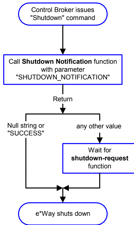
Figure 8 Shutdown functions
