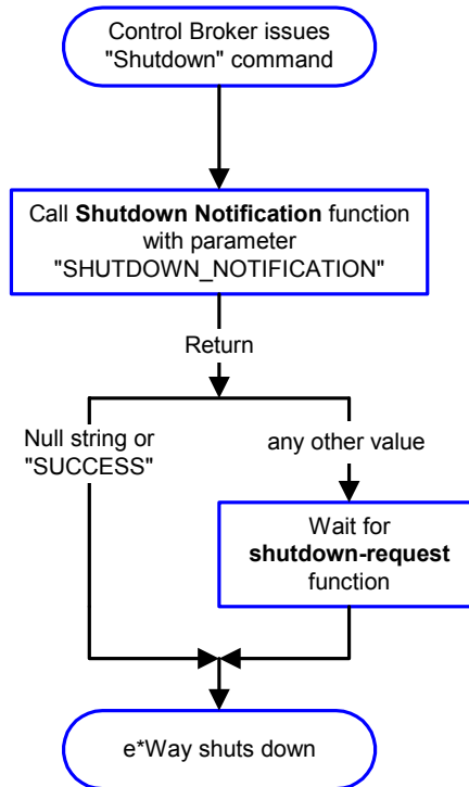
Figure 6 Shutdown Functions
