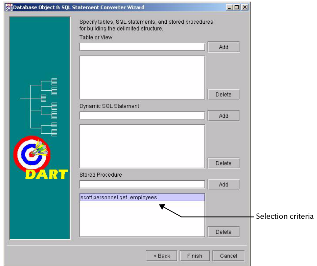
Figure 18 Stored Procedure Selection
