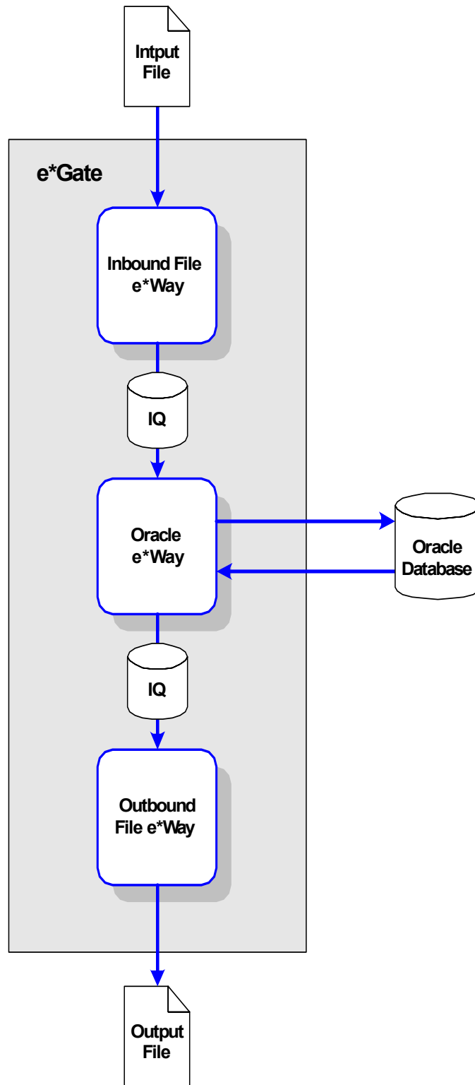
Figure 28 Polling from Oracle Database
