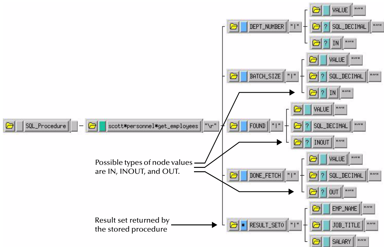
Figure 19 Stored Procedure ETD
