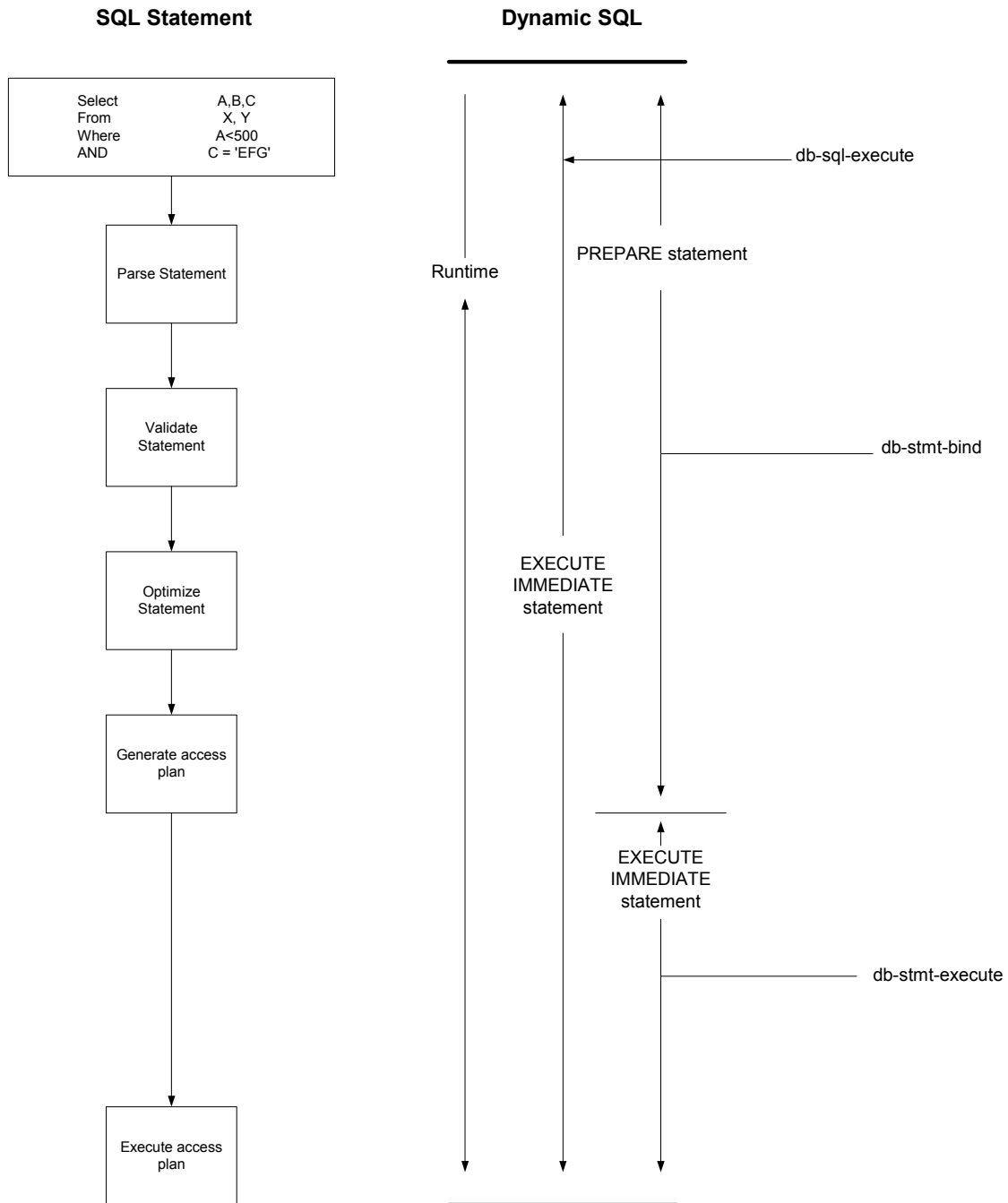
Figure 35 Example of Dynamic SQL Processing
