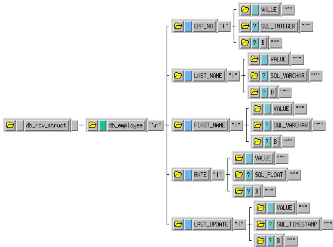
Figure 23 The db_rcv_struct.ssc ETD
