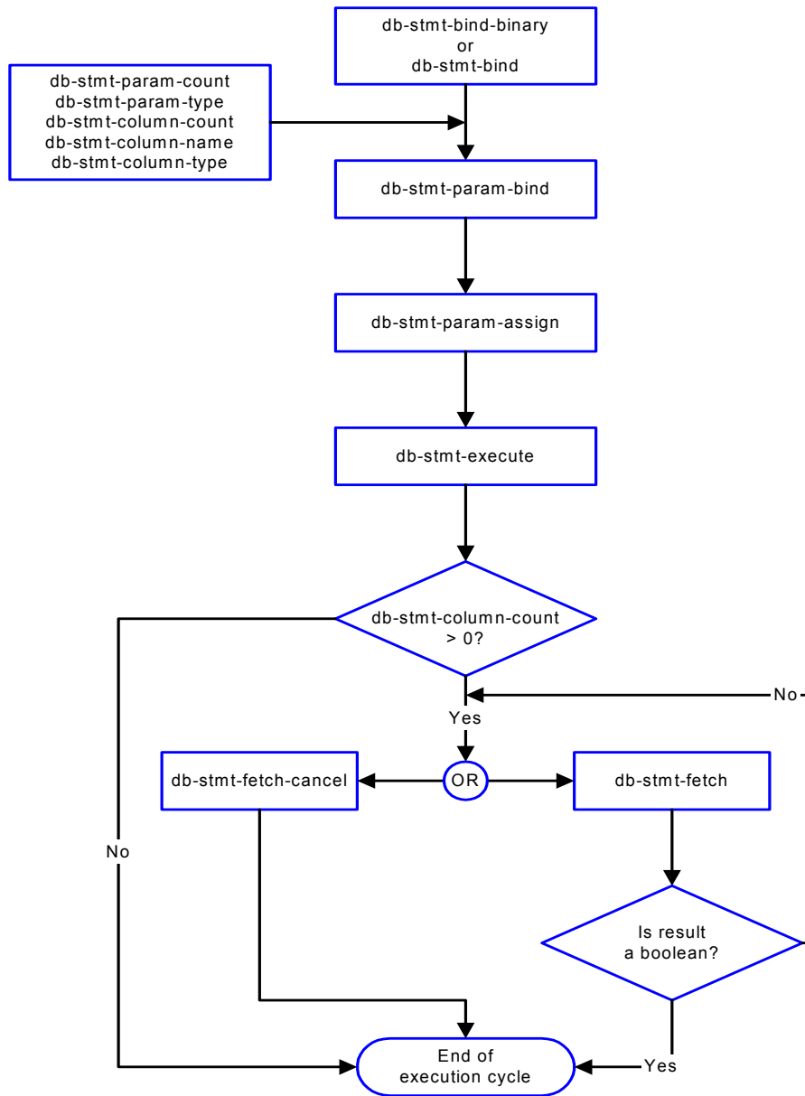
Figure 34 Dynamic Statement Function Flow Chart
