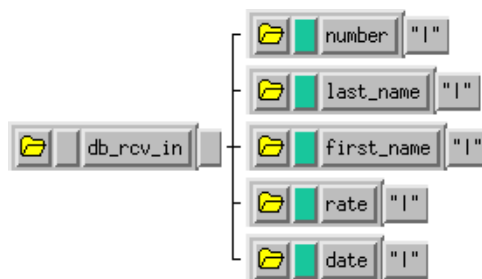
Figure 22 The db_rcv_in.ssc ETD
