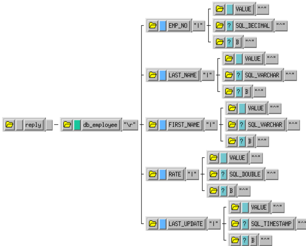
Figure 30 The db_reply.ssc ETD
