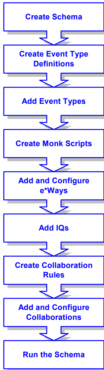
Figure 21 Schema Configuration Steps
