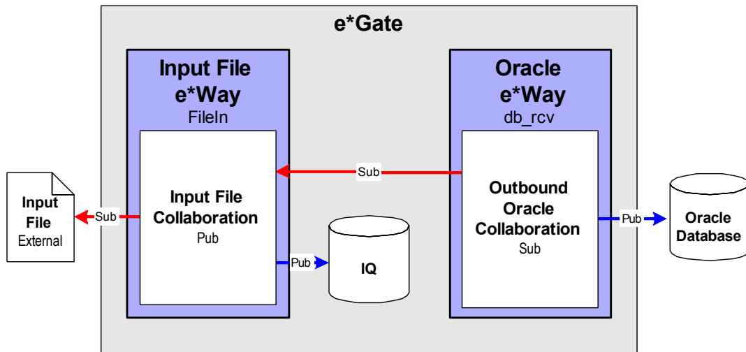
Figure 20 Publishing to Oracle database
