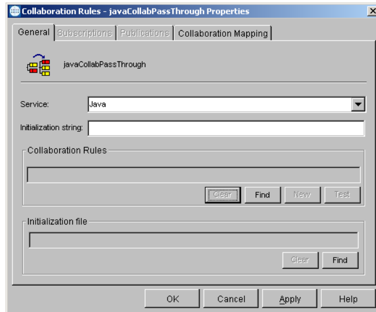
Figure 7 Collaboration Properties
