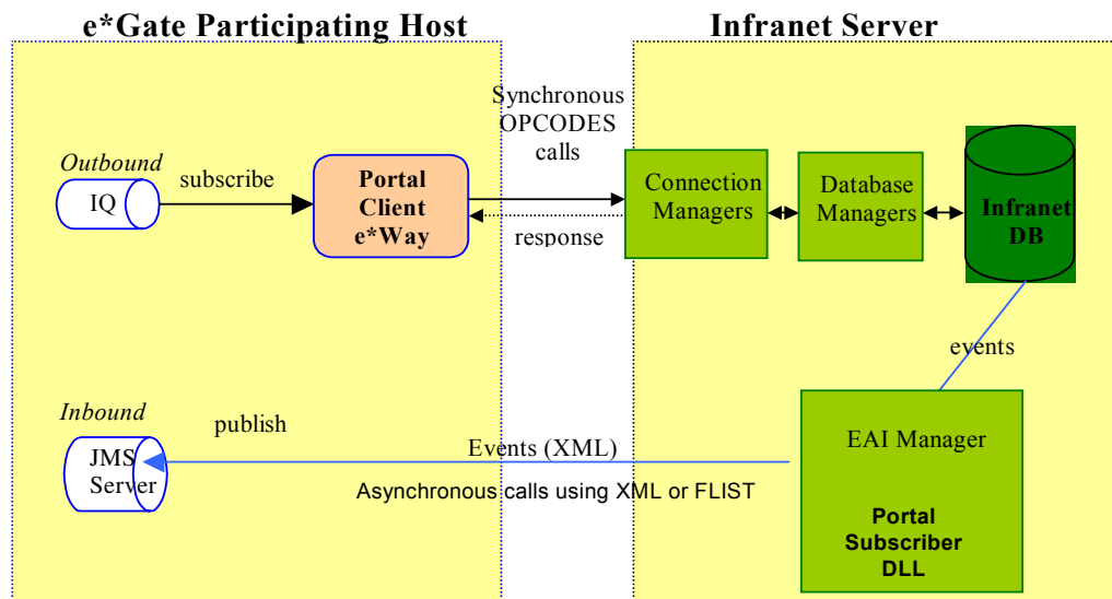
Figure 3 Portal Infranet e*Way System Architecture
