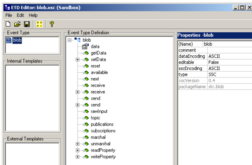
Figure 9 blob.xsc
