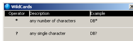
Figure 12 Wildcards
