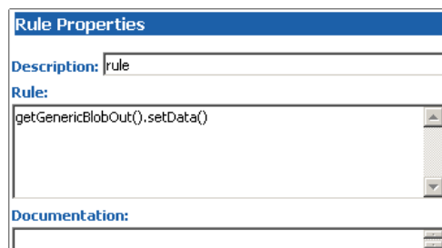
Figure 36 Rule Properties
