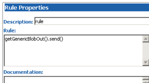
Figure 39 GenericBlobOut send()
