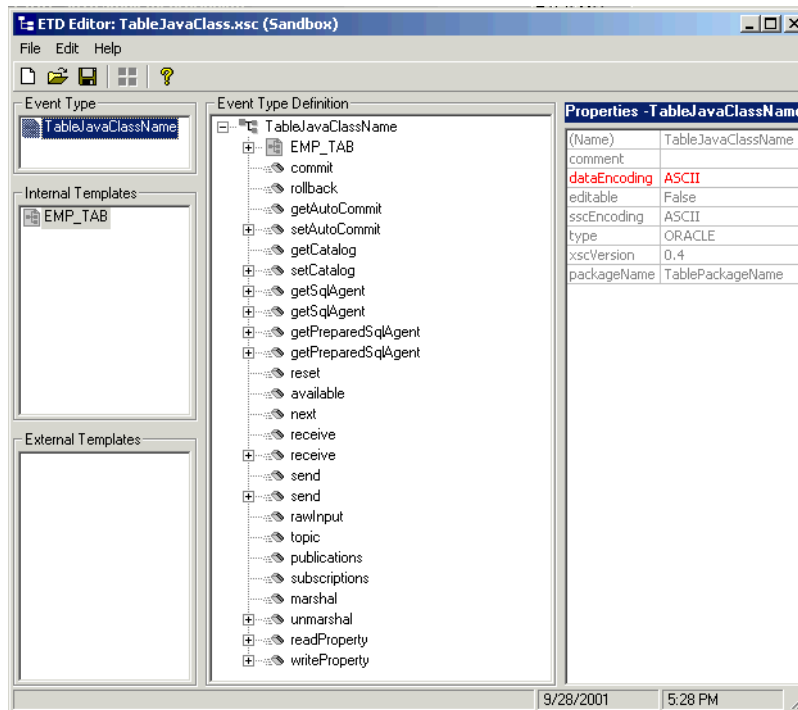
Figure 25 TableJavaClass
