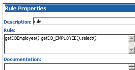
Figure 33 Rule Properties
