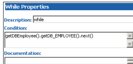
Figure 35 While Properties
