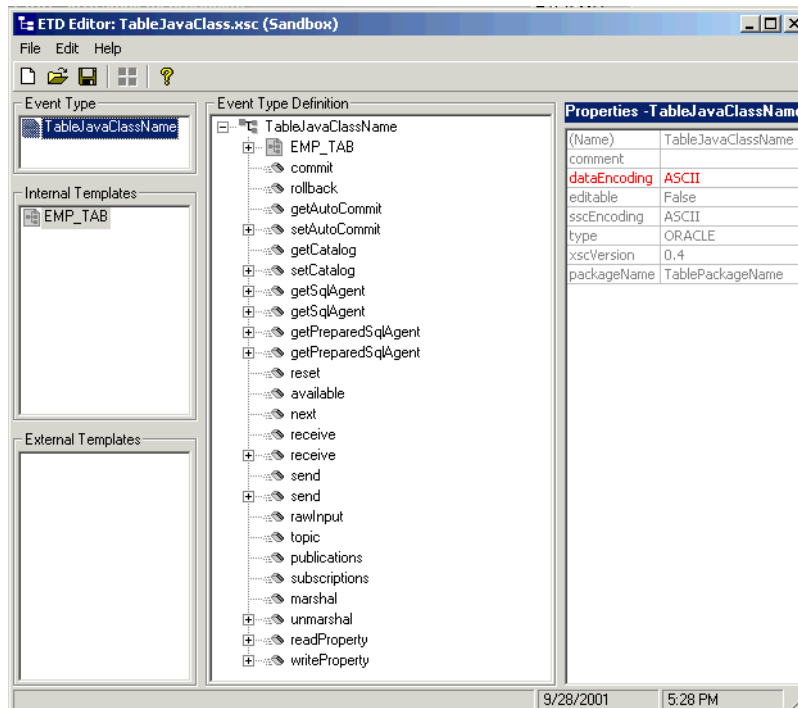
Figure 26 TableJavaClass
