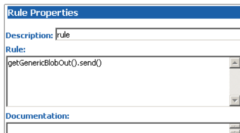
Figure 40 GenericBlobOut send()
