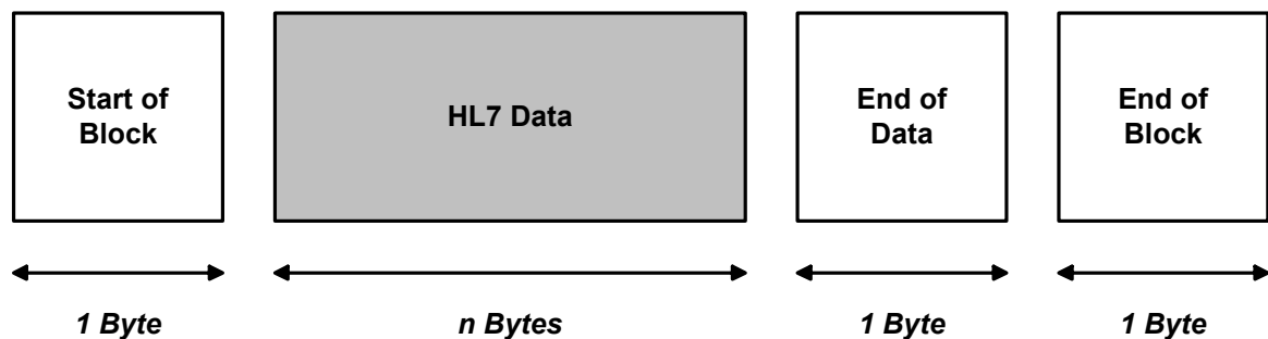
Figure 1 MLLP Envelope Structure
