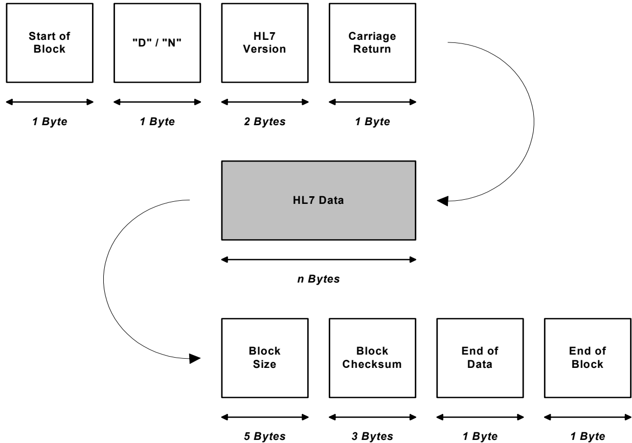
Figure 2 HLLP Envelope Structure
