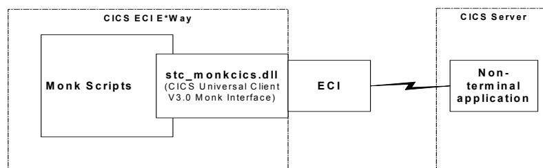
Figure 8 Architectural Overview
