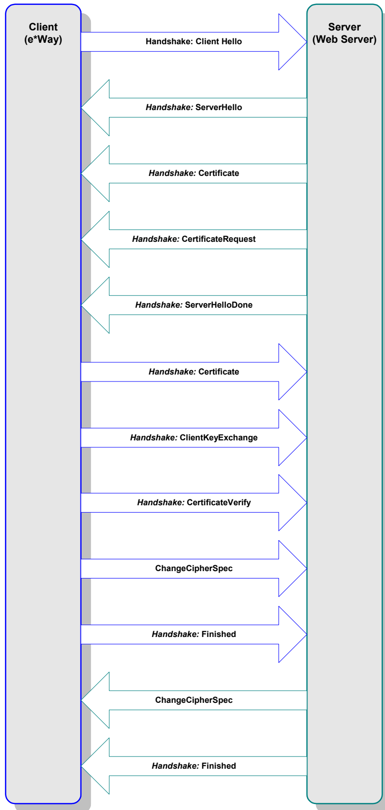
Figure 21 Dual Authentication
