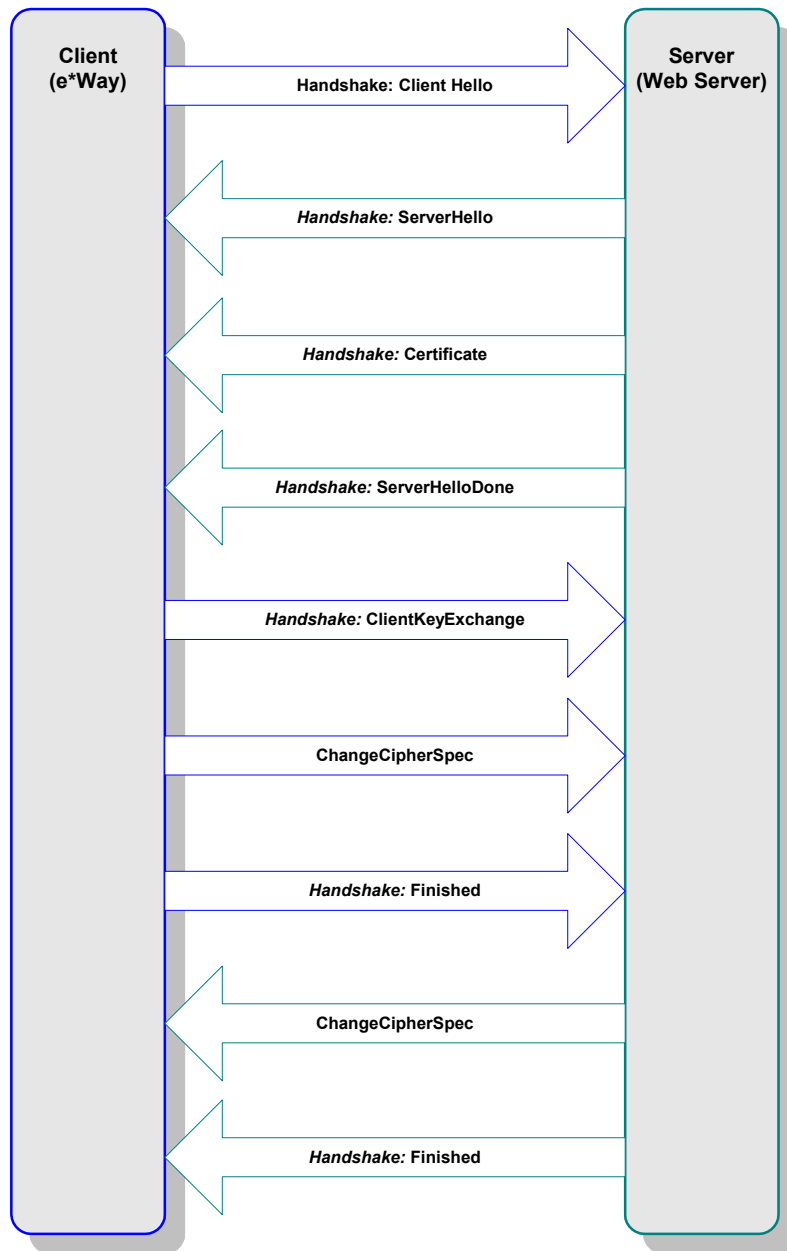
Figure 20 Server-side Authentication
