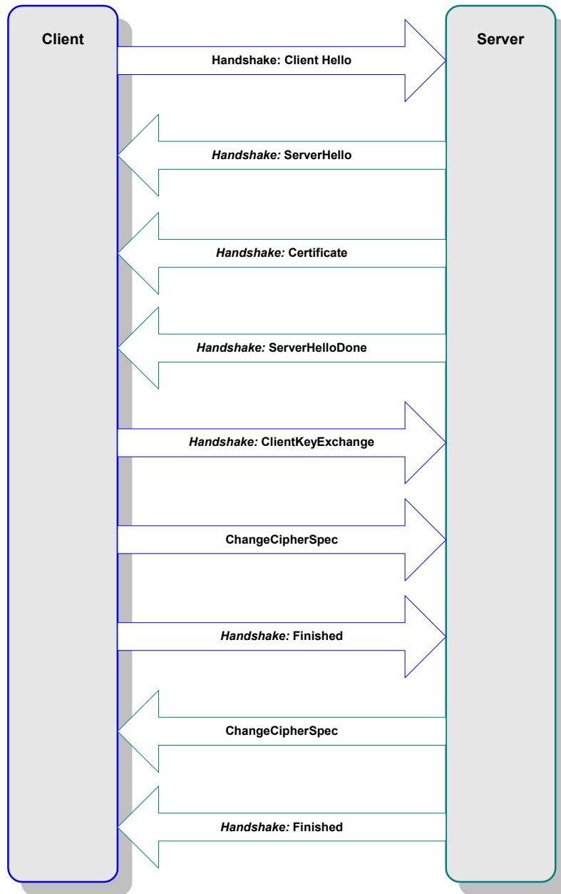
Figure 4 Server-side Authentication
