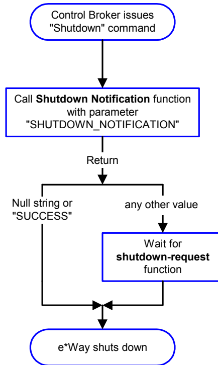
Figure 12 Shutdown Functions
