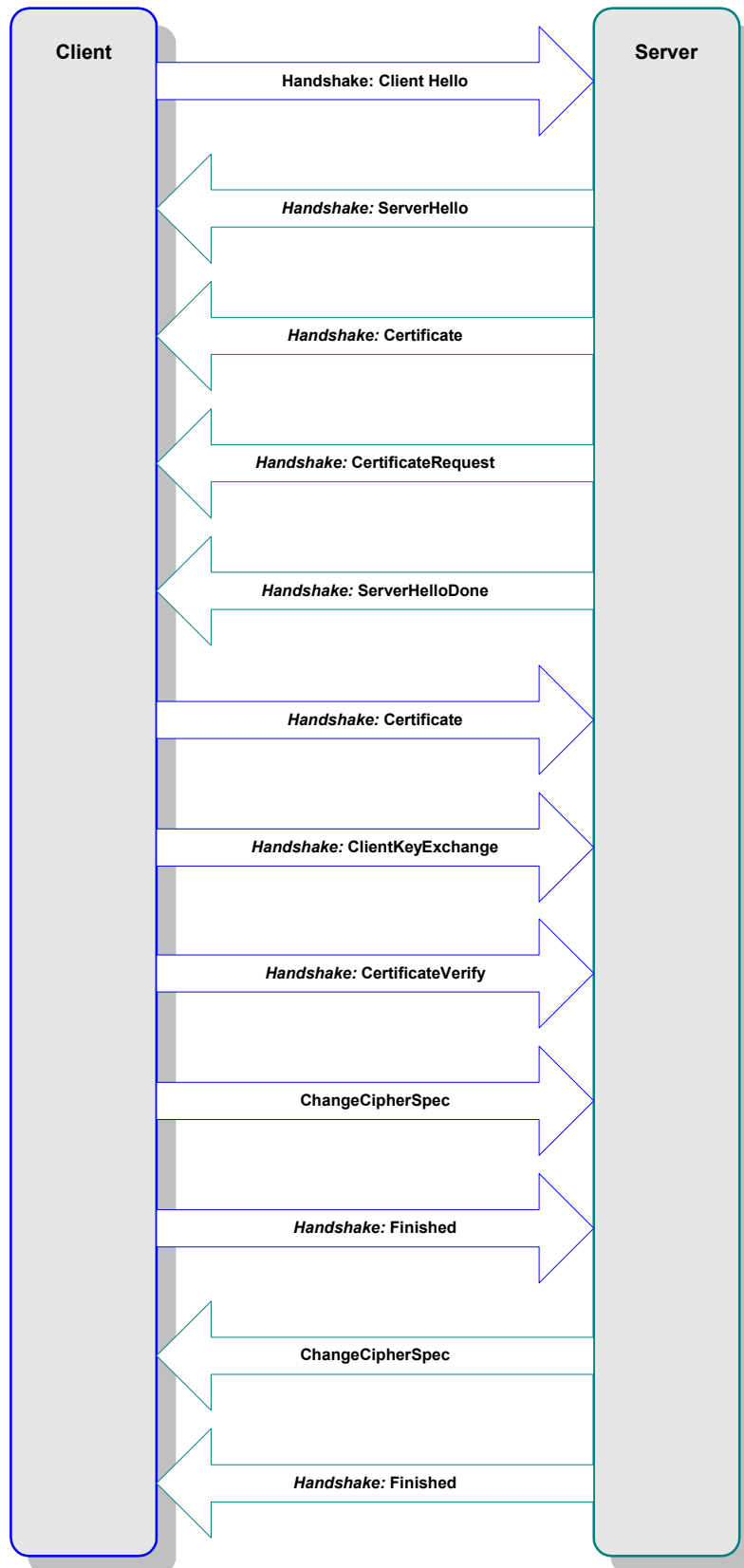
Figure 5 Dual Authentication
