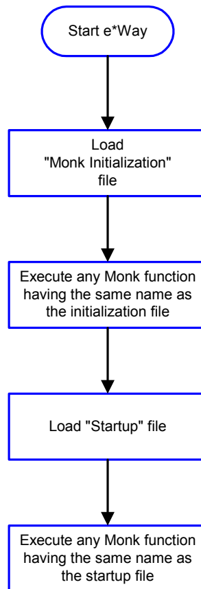
Figure 8 Initialization Functions
