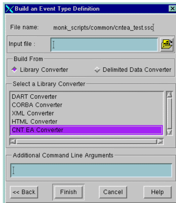
Figure 10 Build an Event Type Definition - Jacada Converter
