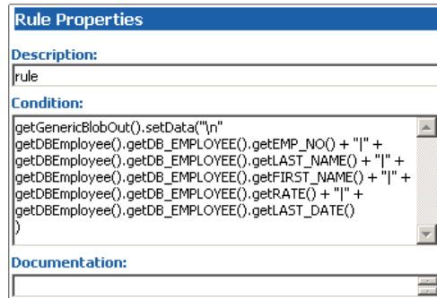
Figure 34 Rule Properties (Continued)
