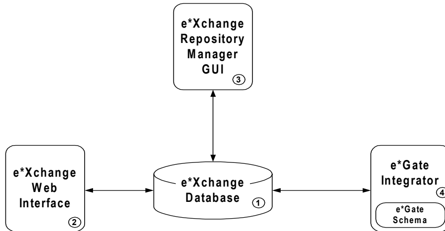
Figure 3 e*Xchange Components
