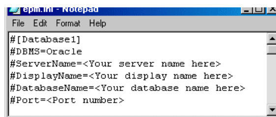
Figure 4 epm.ini File
