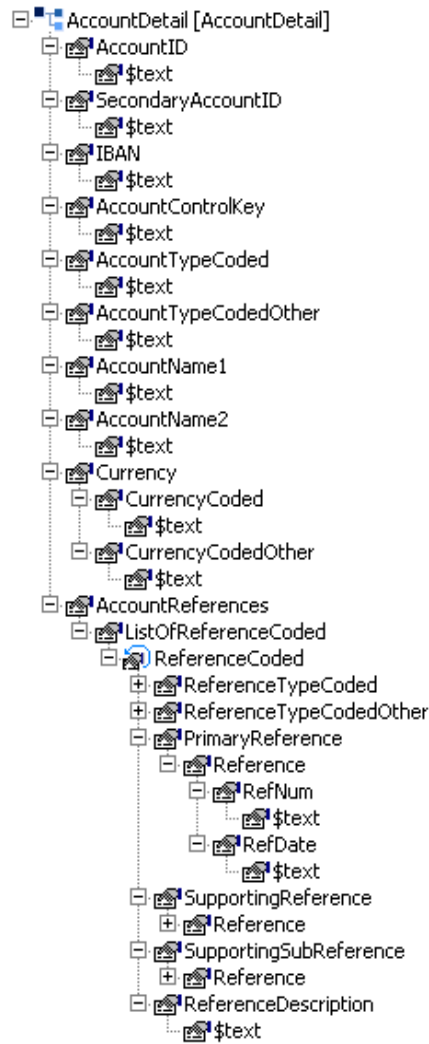
Figure 5 AccountDetail.xsc Components
