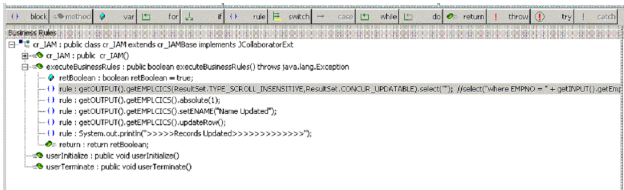
Figure 25 Update() Method Business Rule
