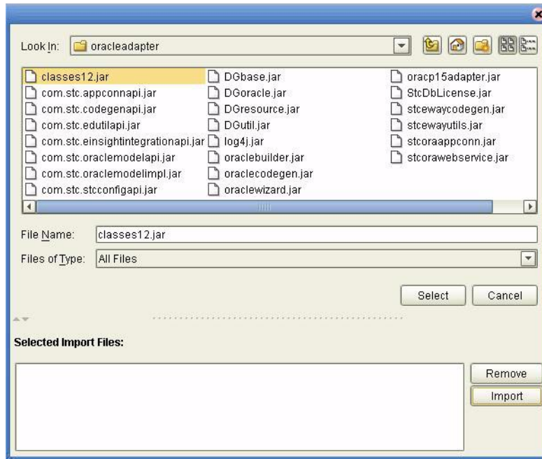
Figure 71 Importing Classes12.jar
