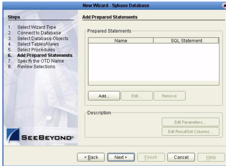
Figure 16 Prepared Statement
