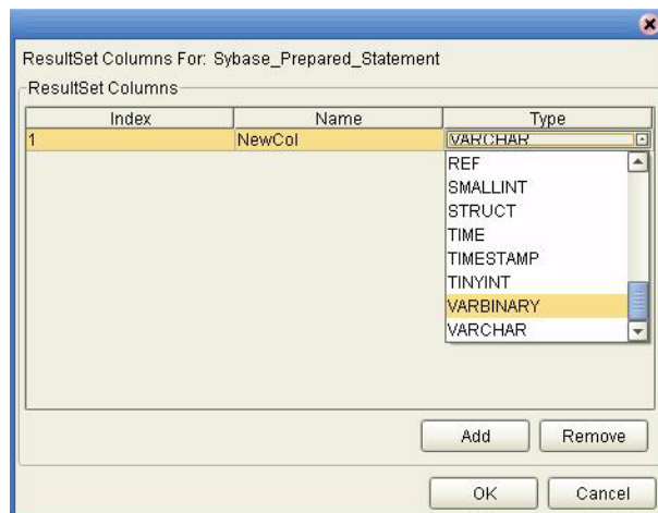
Figure 19 ResultSet Columns
