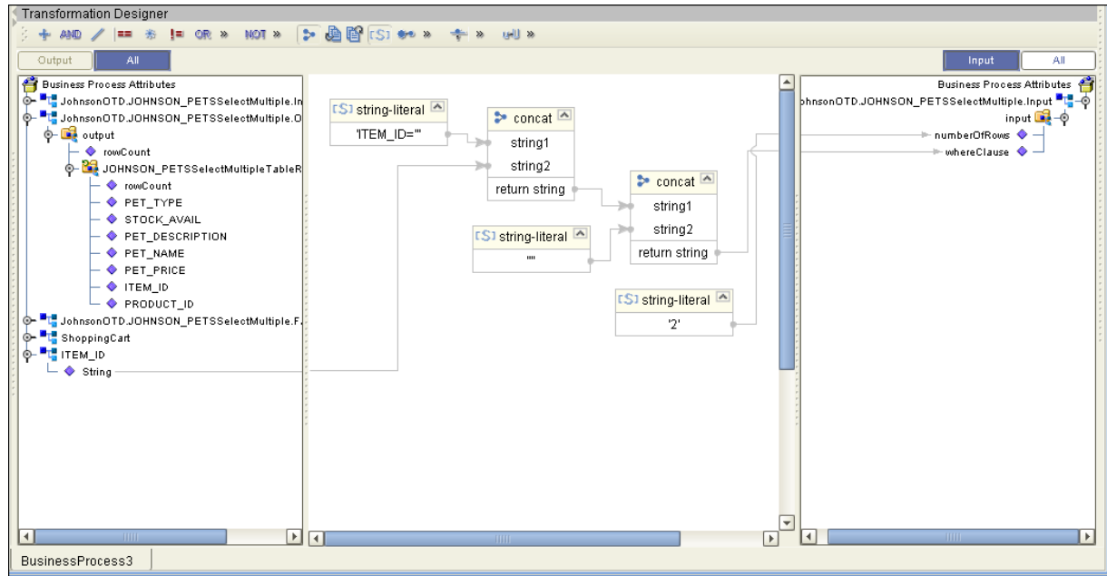
Figure 28 SelectMultiple Input
