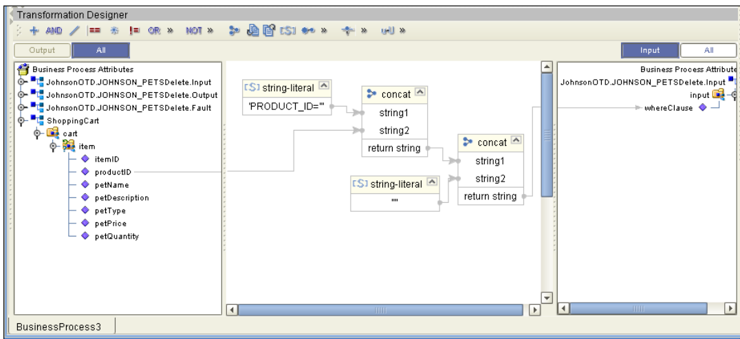
Figure 40 Delete Input
