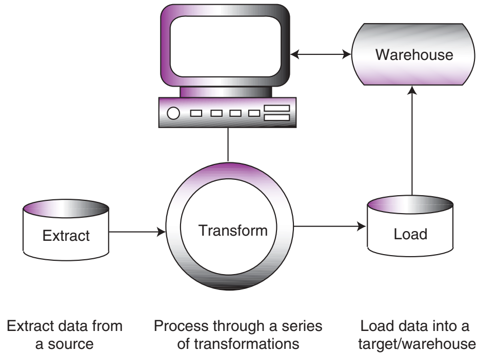
Figure 31 The ETL Process
