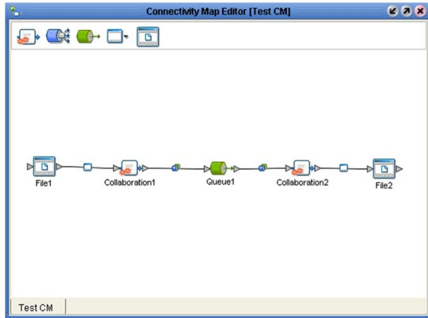
Figure 7 Connectivity Map Editor
