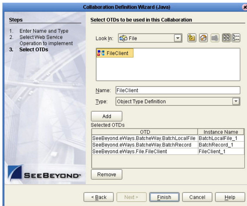
Figure 48 Collaboration Definition Wizard (Java) - Select OTDs
