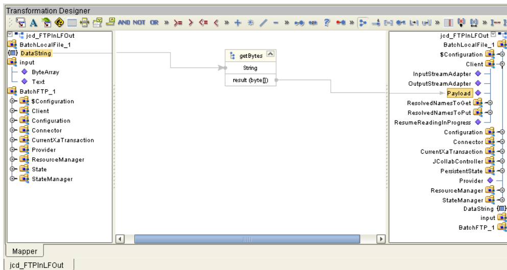
Figure 40 Collaboration Editor (Java) - Transformation Designer
