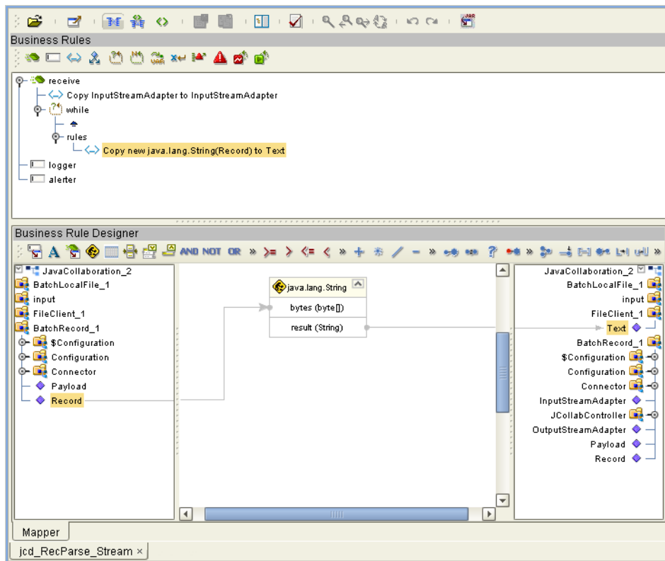
Figure 51 Collaboration Editor (Java) - Business Rules
