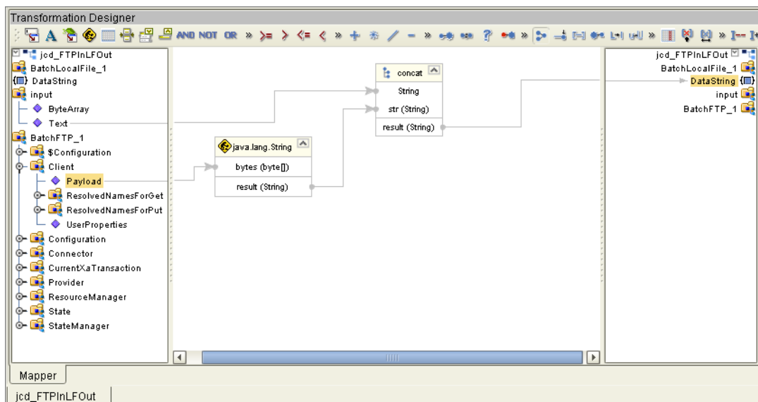
Figure 39 Collaboration Editor (Java) - Transformation Designer
