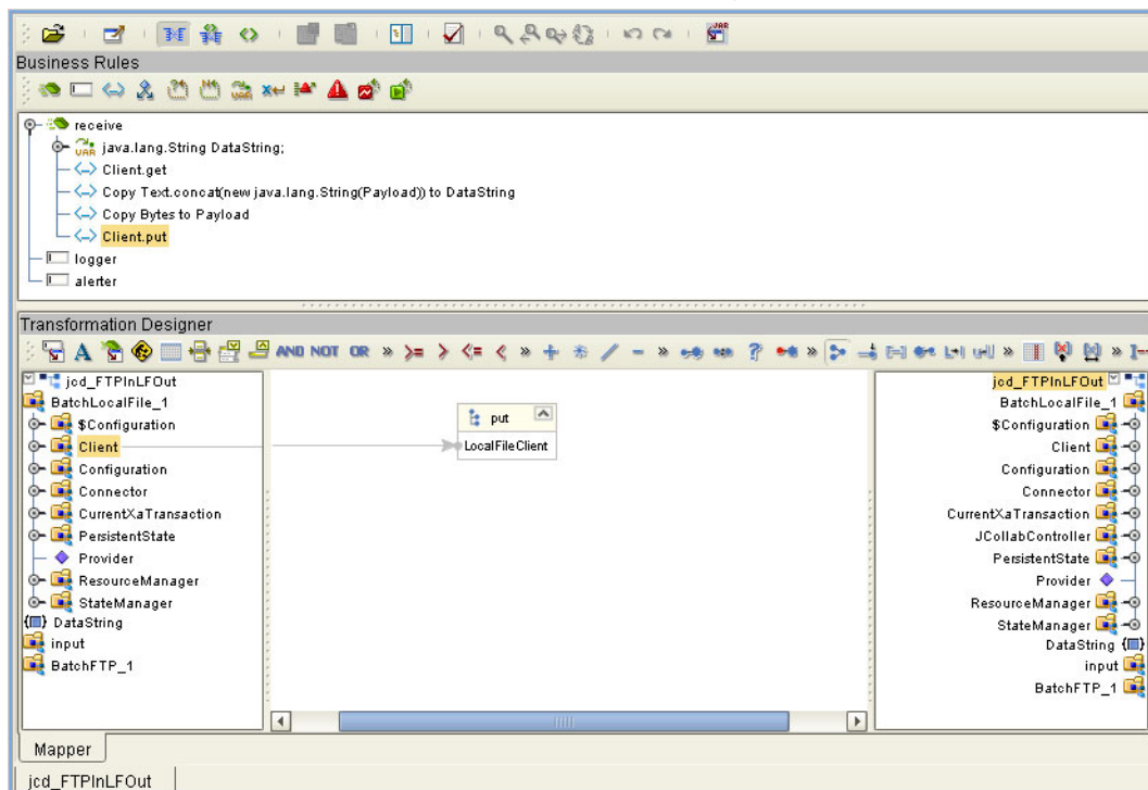
Figure 41 Collaboration Editor (Java) - Creating Business Rules
