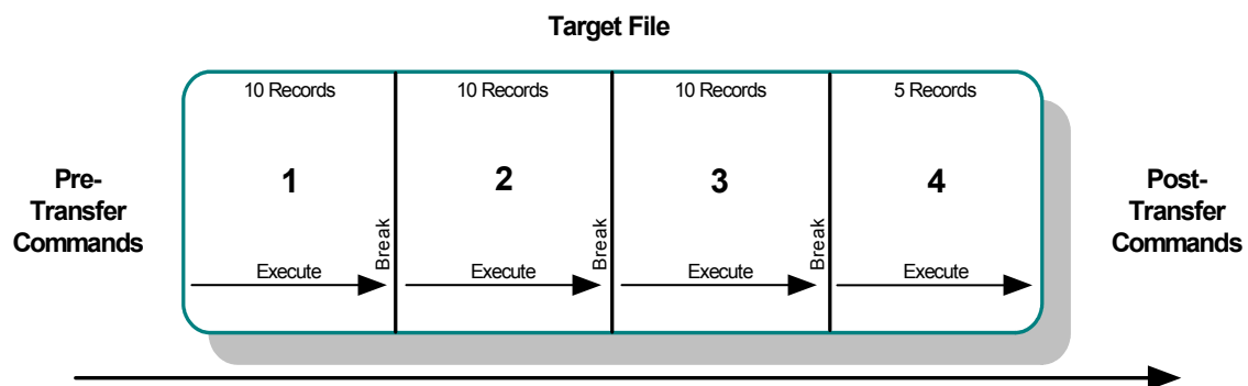
Figure 55 Resume Reading Operation
