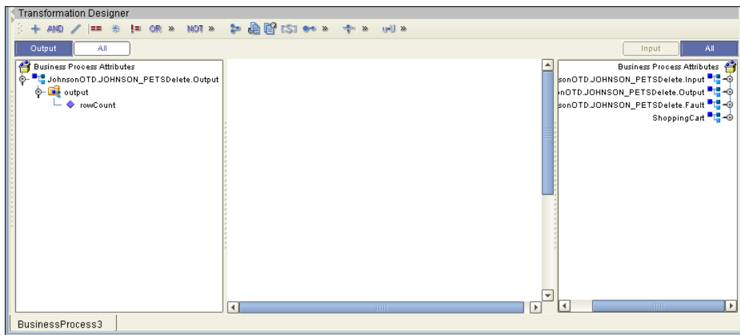
Figure 41 Delete Output
