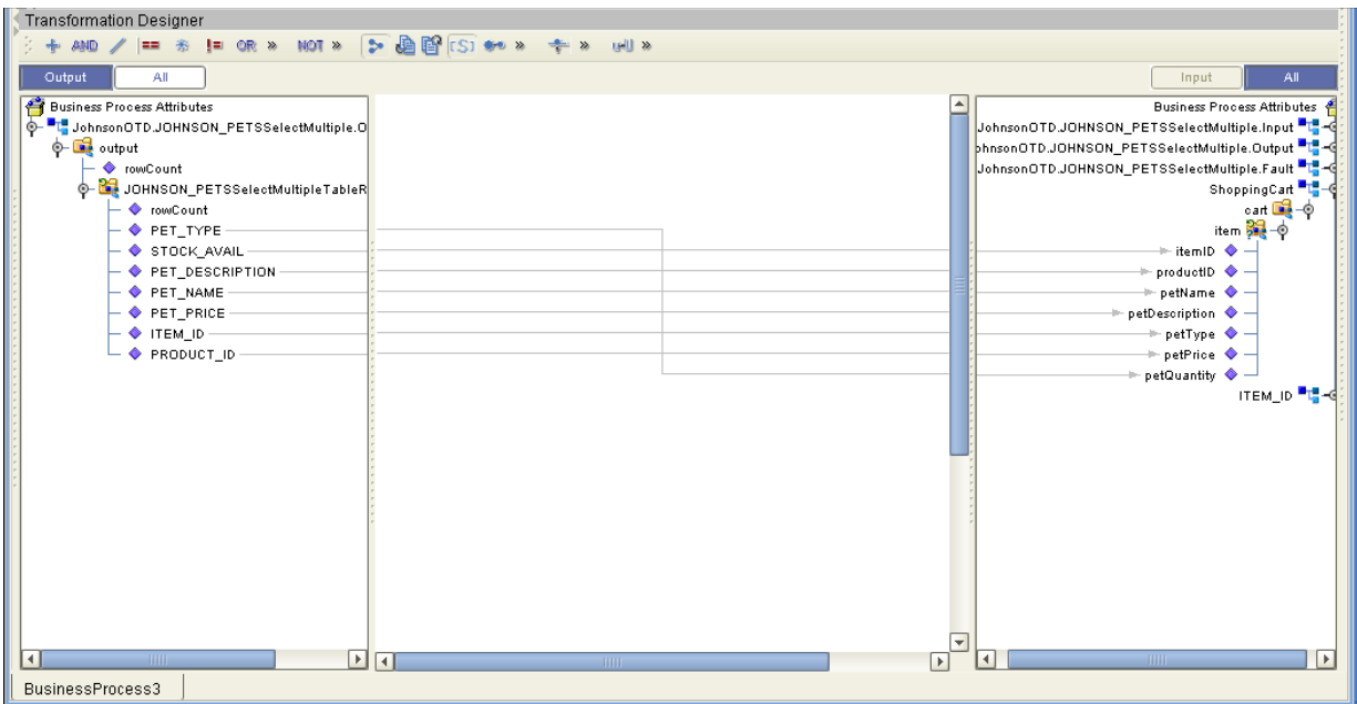
Figure 29 SelectMultiple Output
