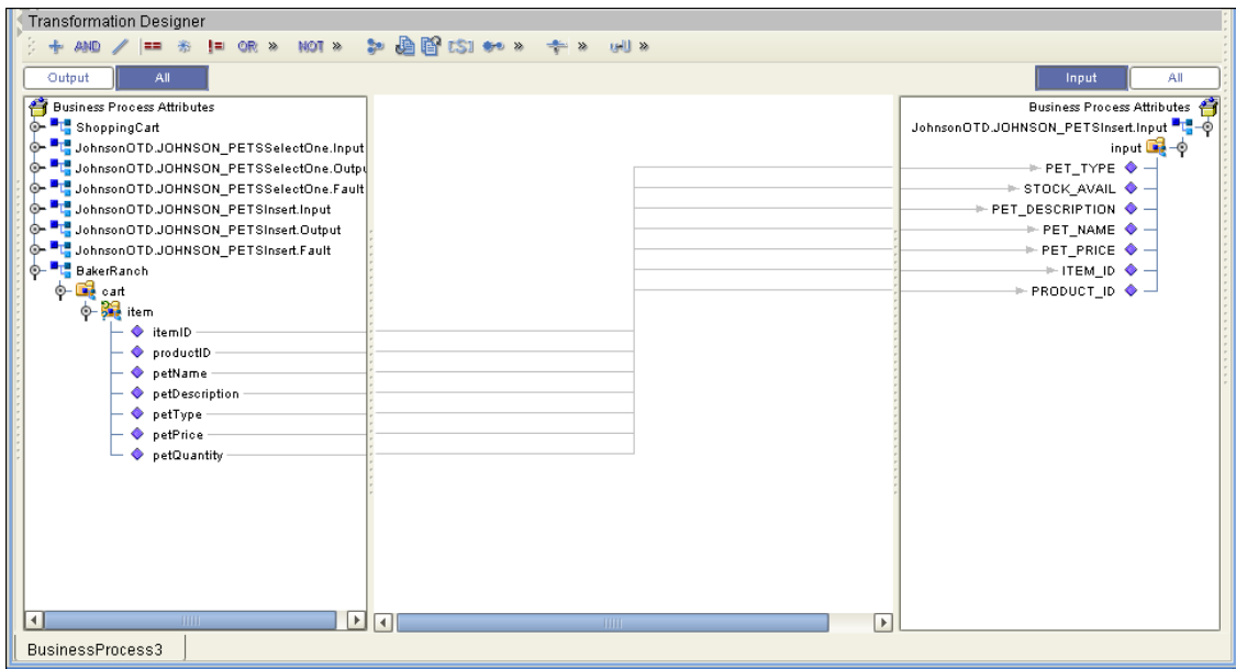
Figure 34 Insert Input
