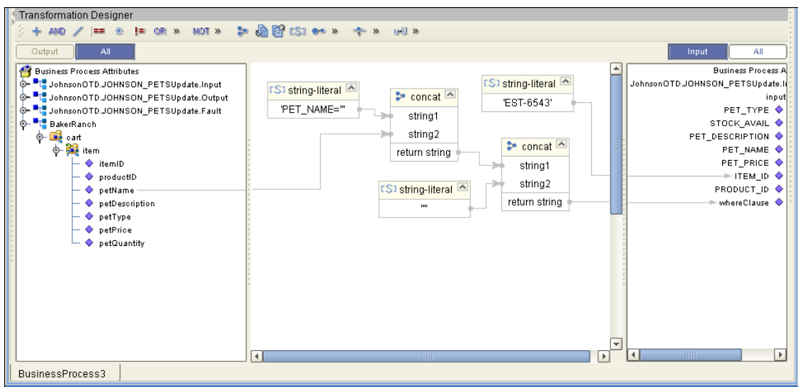
Figure 37 Update Input
