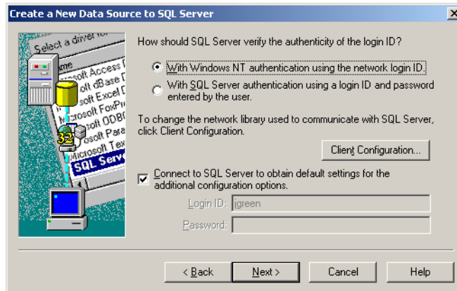
Figure 27 Login Settings
