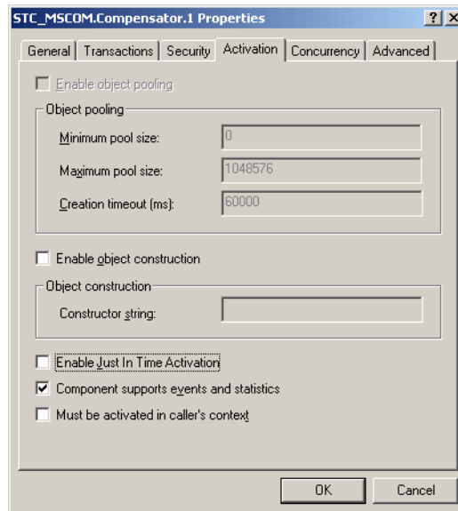
Figure 12 STC_MSCOM.Compenstator Properties:Activation
