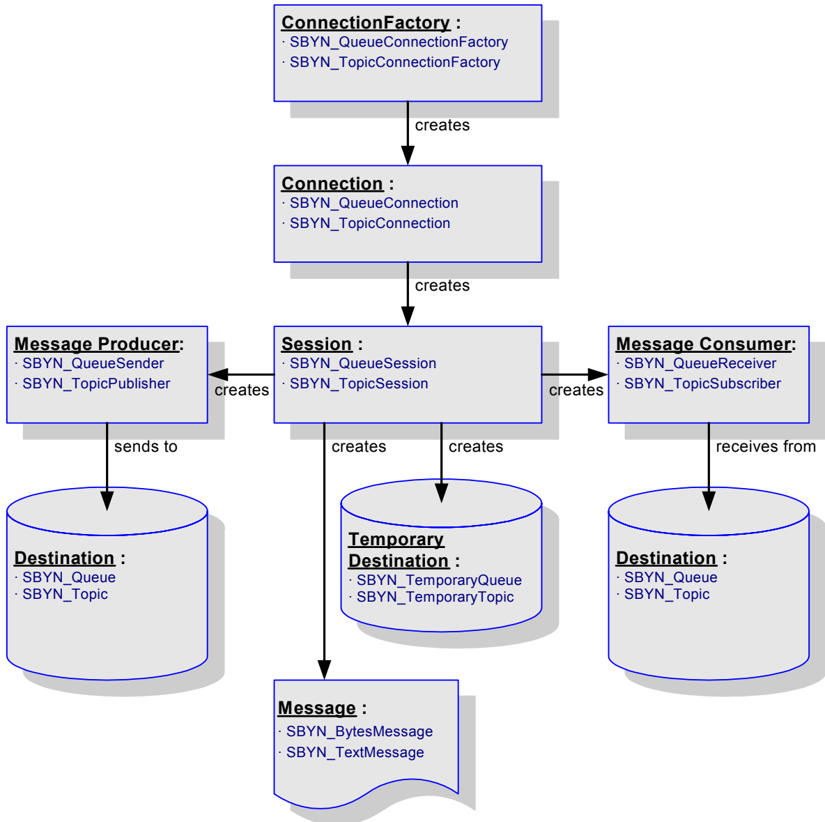
Figure 30 JMS C Object Model
