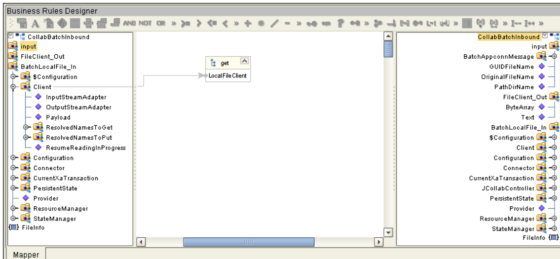
Figure 58 Business Rules Designer - Get file
