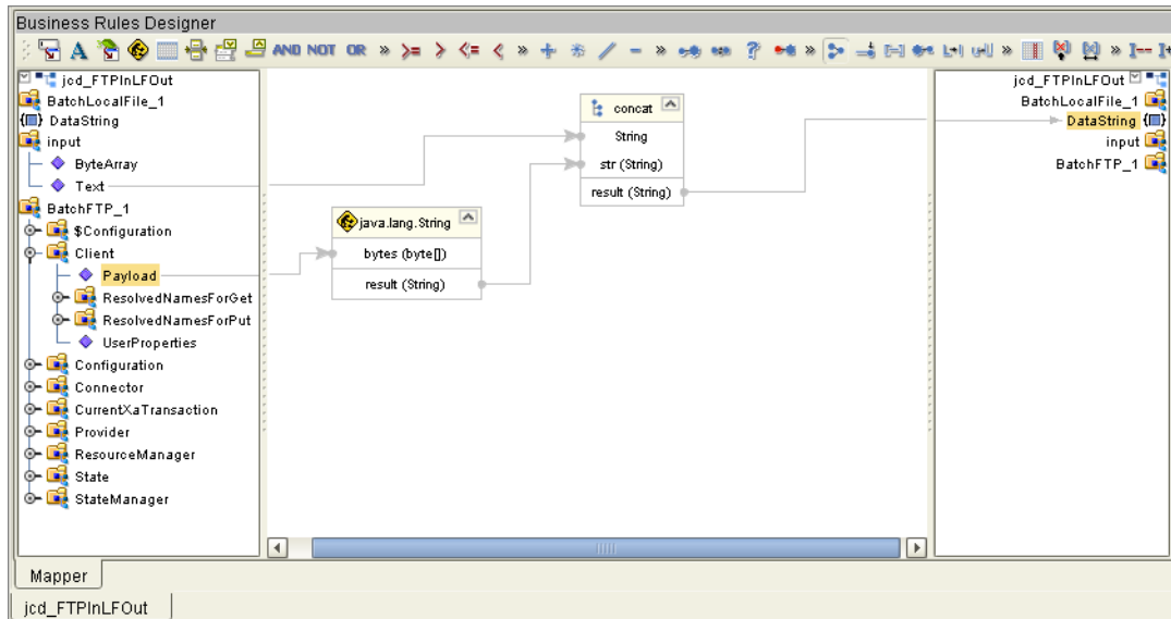
Figure 39 Collaboration Editor (Java) - Business Rules Designer
