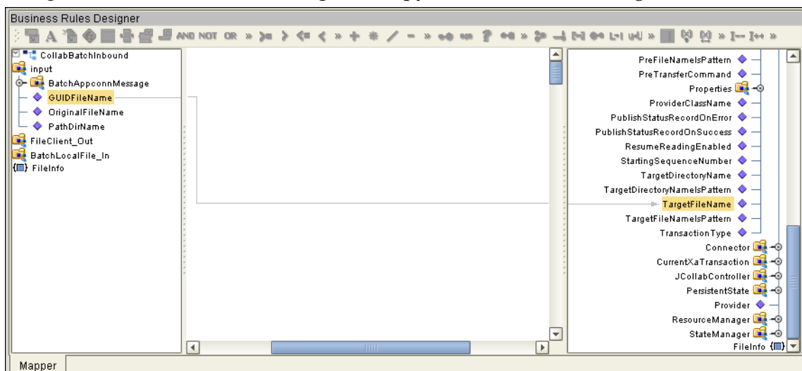
Figure 57 Business Rules Designer - Copy GUIDFileName to TargetFileName
