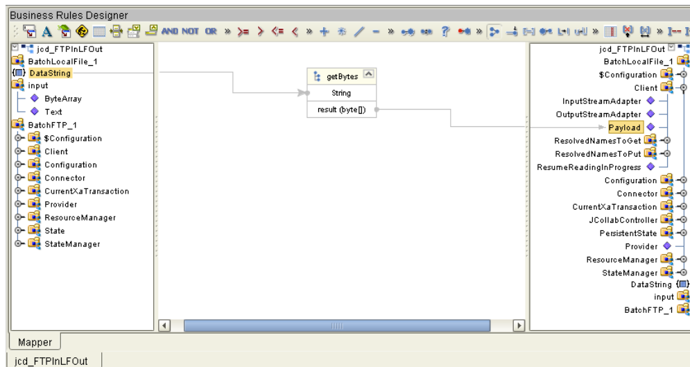
Figure 40 Collaboration Editor (Java) - Business Rules Designer
