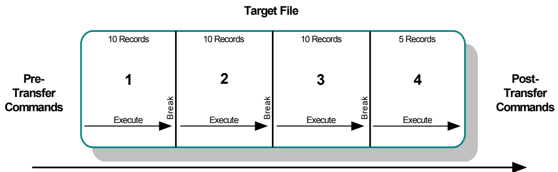
Figure 63 Resume Reading Operation
