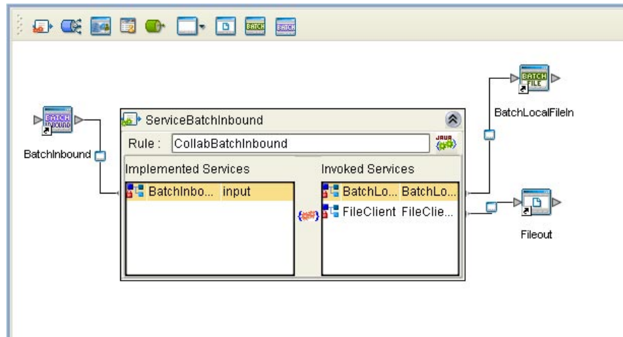
Figure 61 Connectivity Map - Connecting the Project's Components
