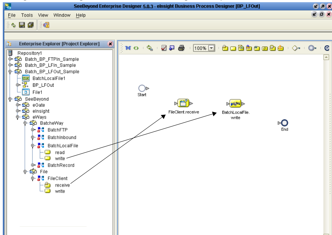
Figure 24 eInsight Business Process Designer - Populate the Canvas
