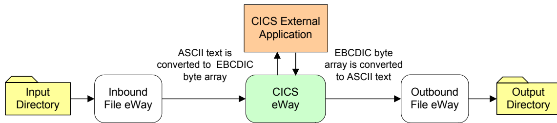
Figure 24 CICS_BP_Sample Project
