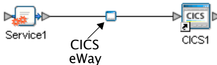
Figure 22 eWay Location.
