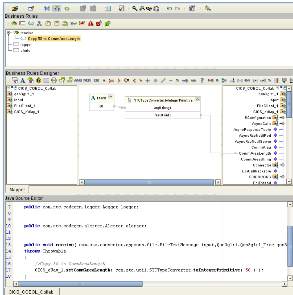
Figure 59 Copy 50 to CommAreaLength Business Rule
