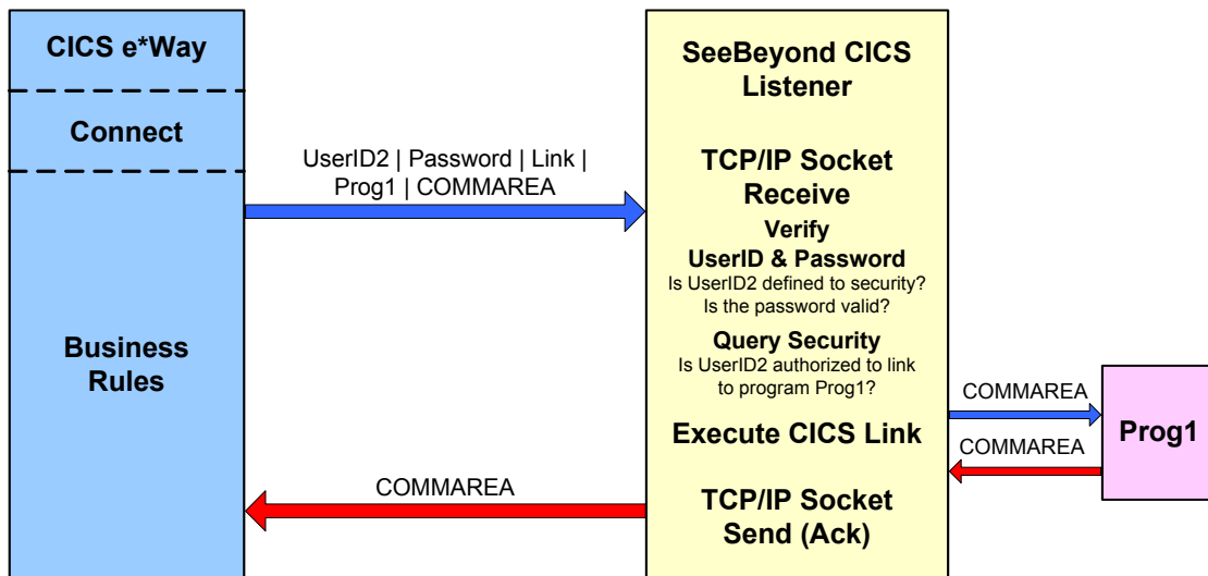
Figure 3 Business Rules Request to Program
