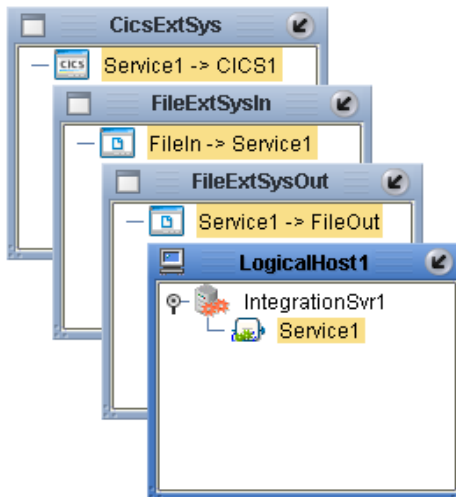
Figure 38 Deployment Profile
