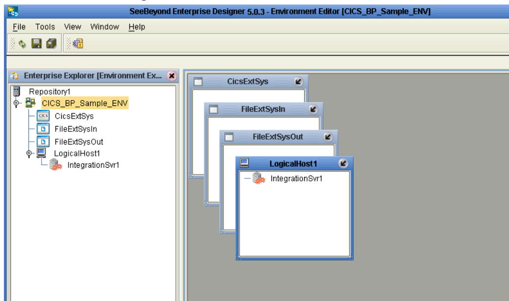
Figure 36 Environment Editor
