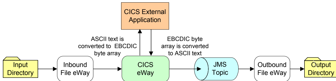
Figure 39 CICS_JCE_Sample Project
