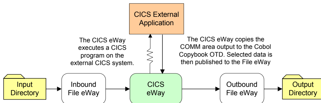
Figure 55 CICS_Cobol_Sample Project
