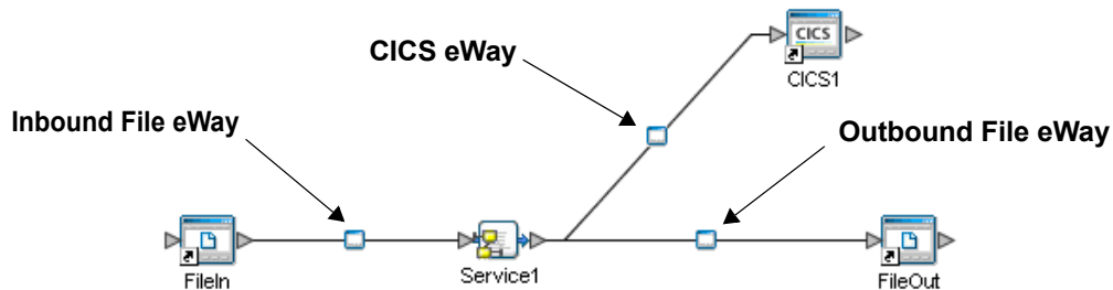
Figure 37 eWays
