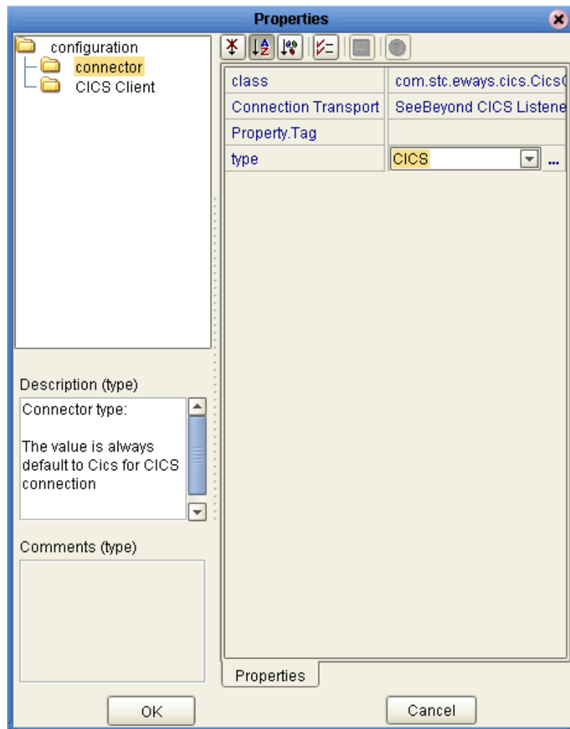
Figure 23 Properties Sheet -- CICS Properties
