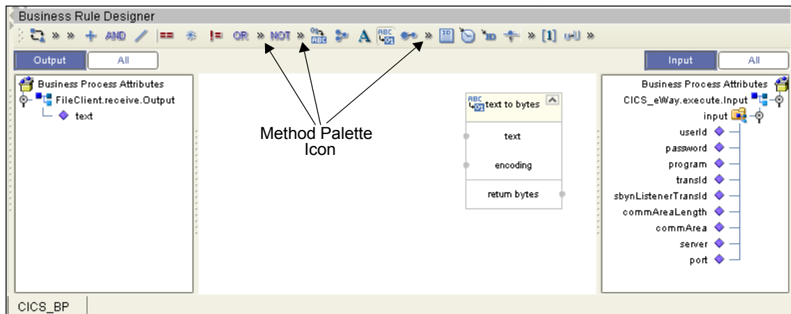
Figure 29 eInsight Business Rule Designer
