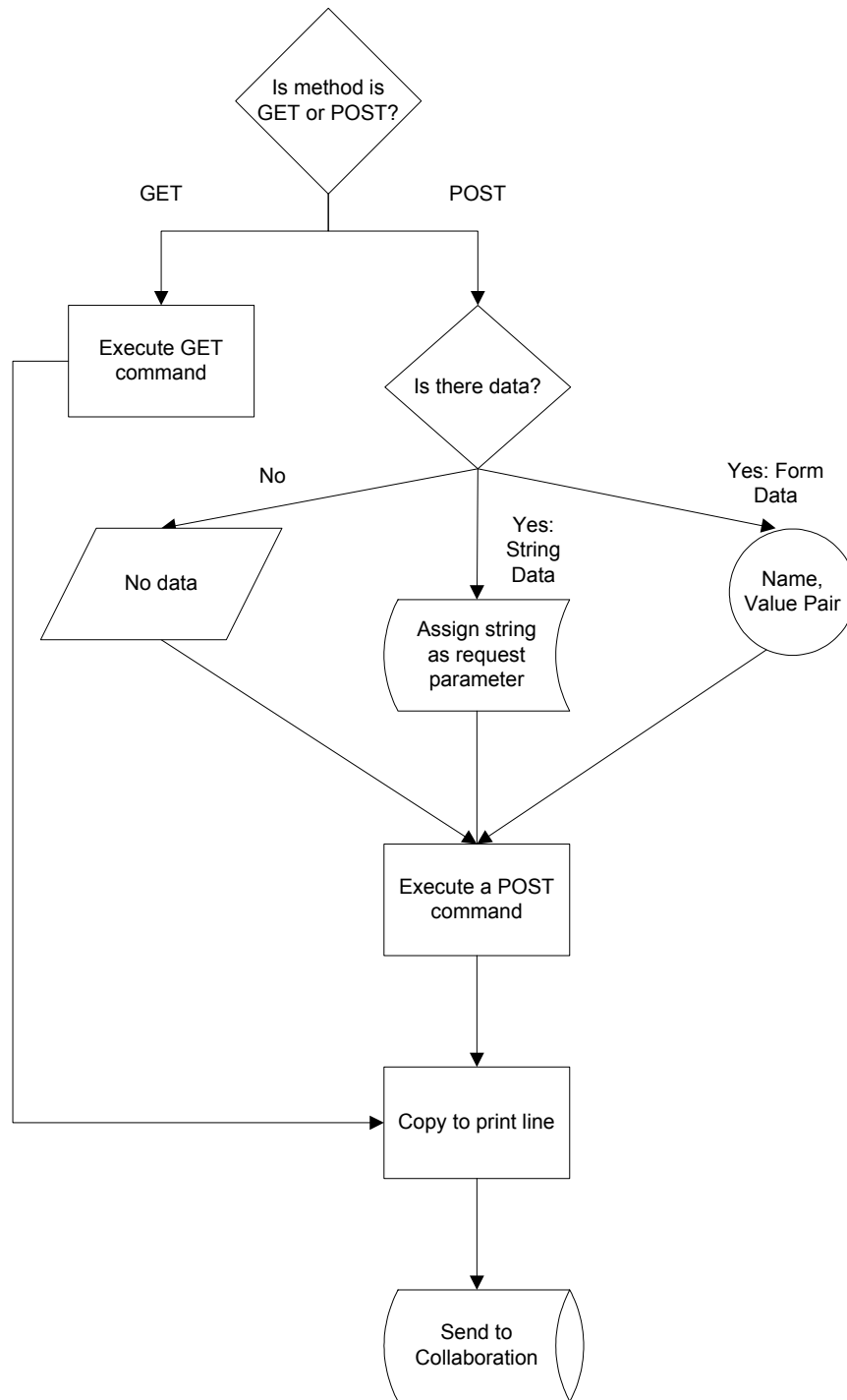
Figure 40 Logic of the Collaboration (Java)
