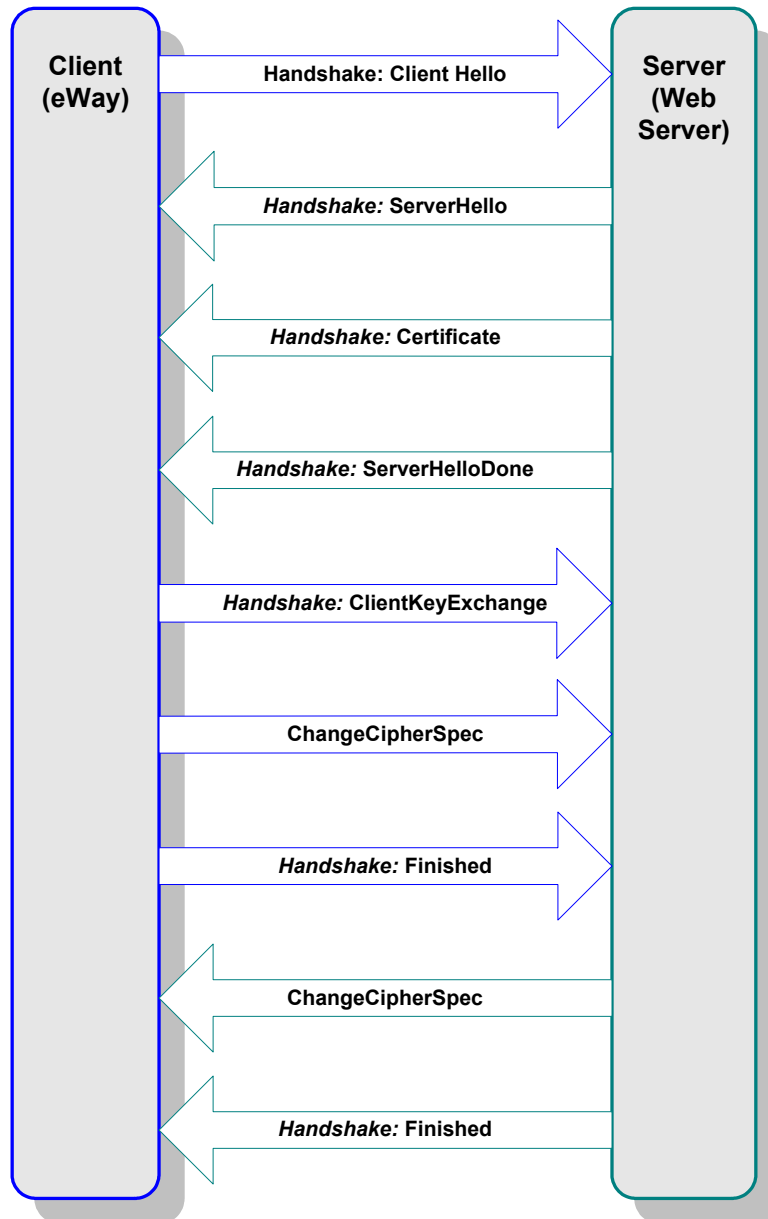
Figure 57 Server-side Authentication
