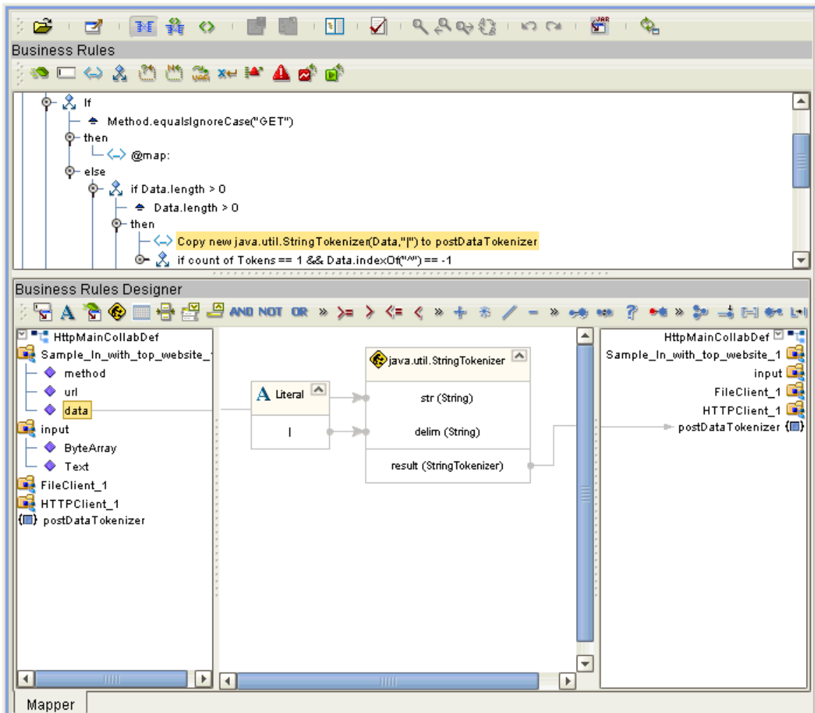
Figure 51 HTTP_JCERule: Collaboration Editor (Java): Creating Business Rules 2
