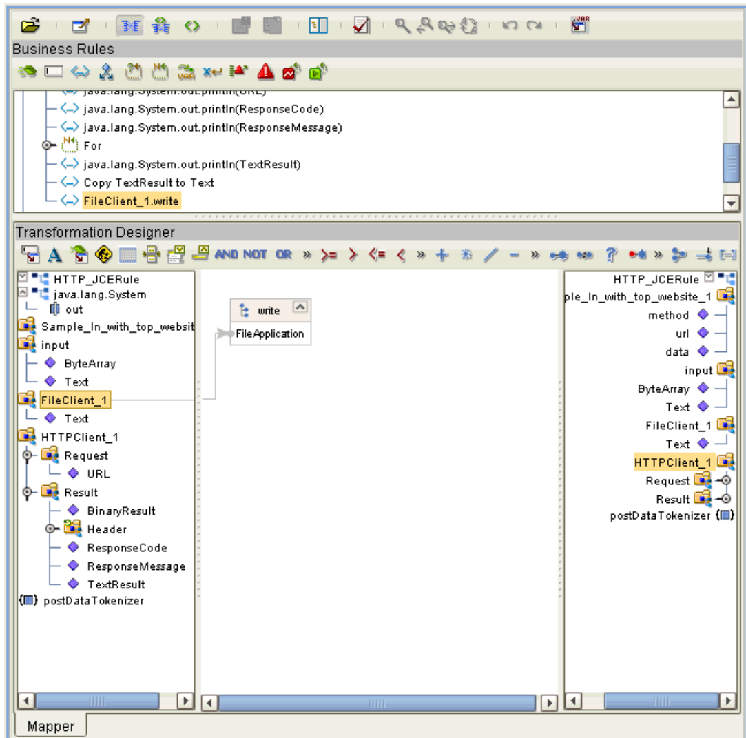
Figure 49 HTTP_JCERule Collaboration Definition: Ninth Business Rule
