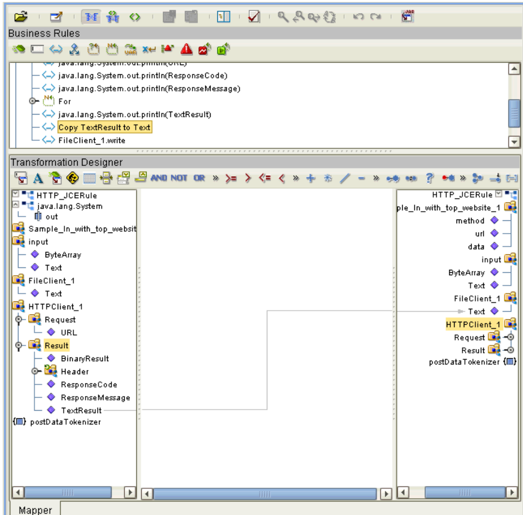
Figure 48 HTTP_JCERule Collaboration Definition: Eighth Business Rule
