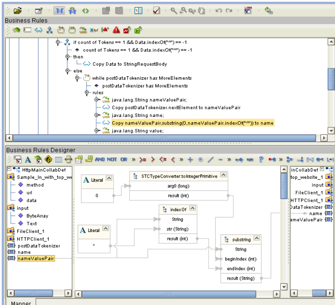
Figure 53 HTTP_JCERule: Collaboration Editor (Java): Creating Business Rules 4
