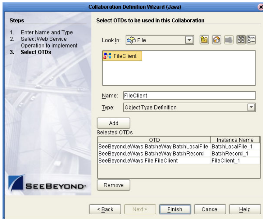
Figure 67 Collaboration Definition Wizard (Java) - Select OTDs
