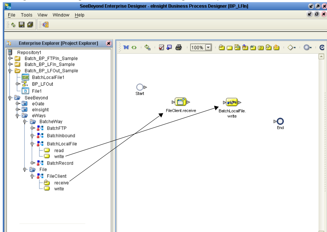
Figure 44 eInsight Business Process Designer - Populate the Canvas
