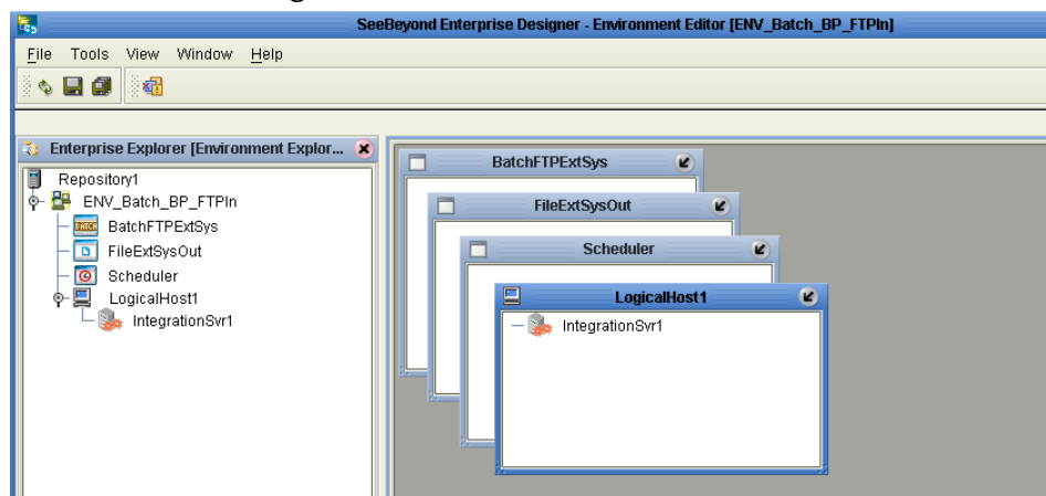
Figure 34 Environment Editor
