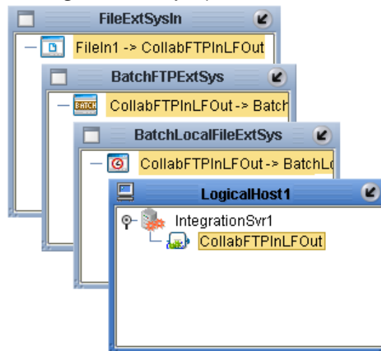
Figure 65 Deployment Profile
