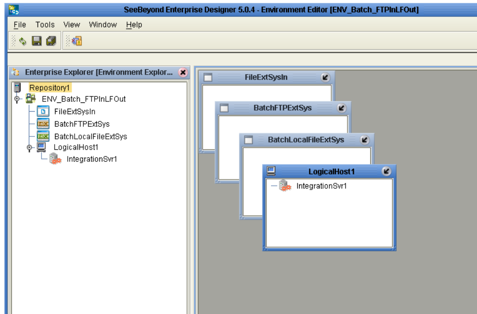
Figure 62 Environment Editor
