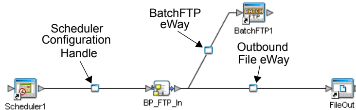
Figure 35 eWay Configurations
