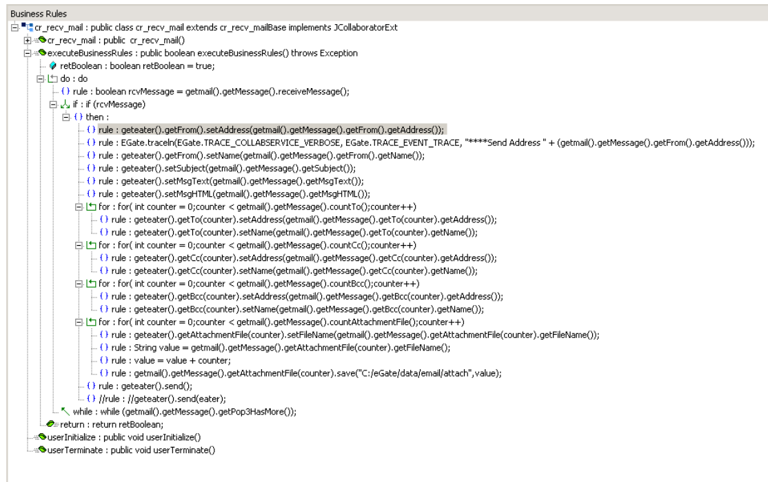
Figure 20 Business Rules - Receiving Collaboration
