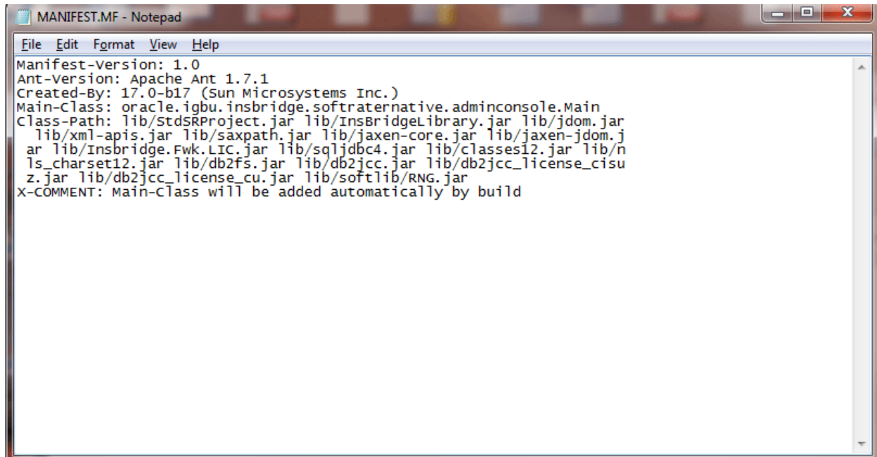
Figure 27 Adding a SoftLibrary Outside the Console
