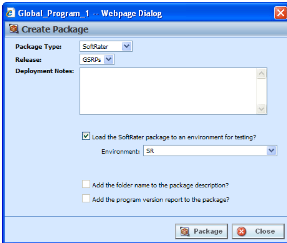
Figure 225 Creating a Global Versioning Package
