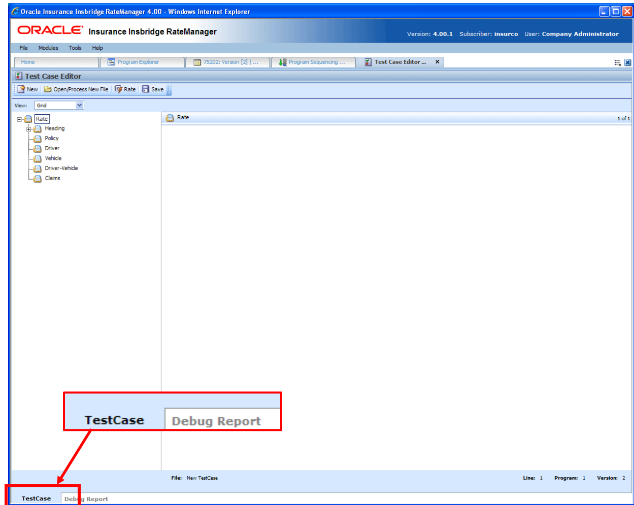
Figure 229 Test Program Tab
