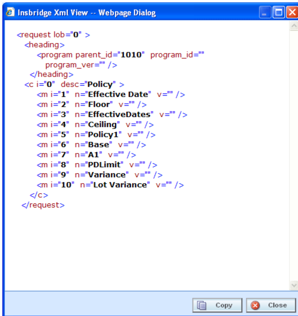
Figure 327 Workflow Inputs XML
