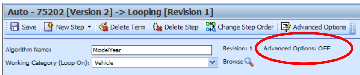
Figure 156 Adding an Advanced Option to a Rating Algorithm
