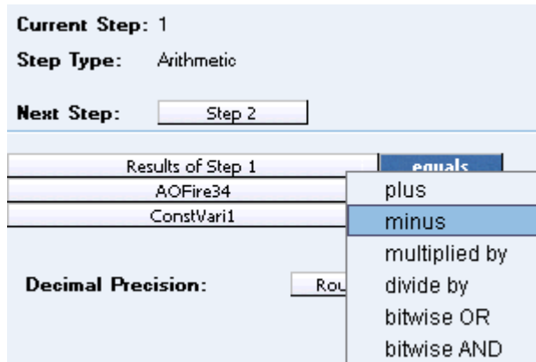
Figure 107 Setting an Arithmetic Step 2
