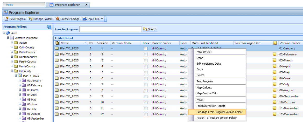
Figure 52 Unassigning a Program Version
