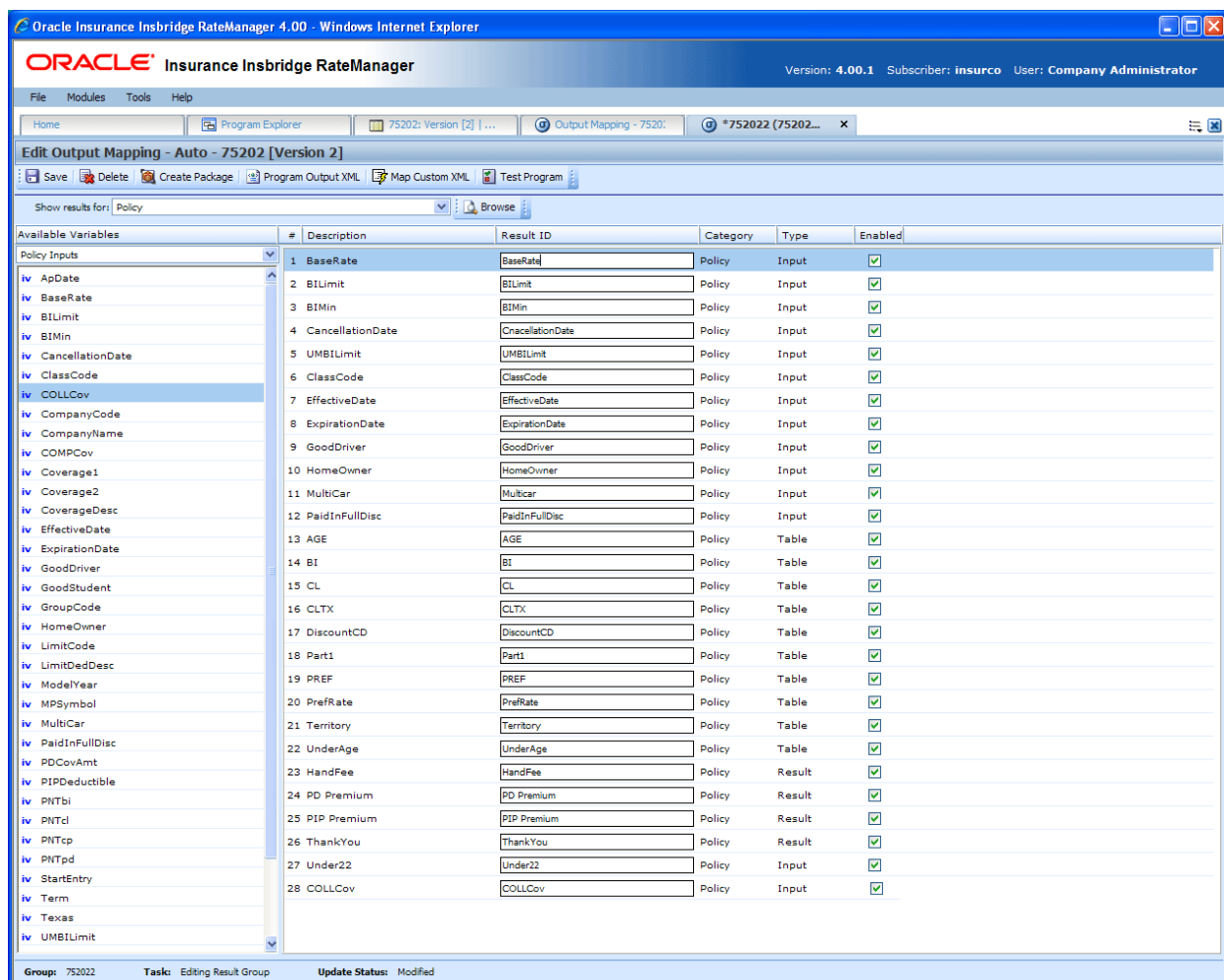
Figure 207 Adding Variables to Output Mapping
