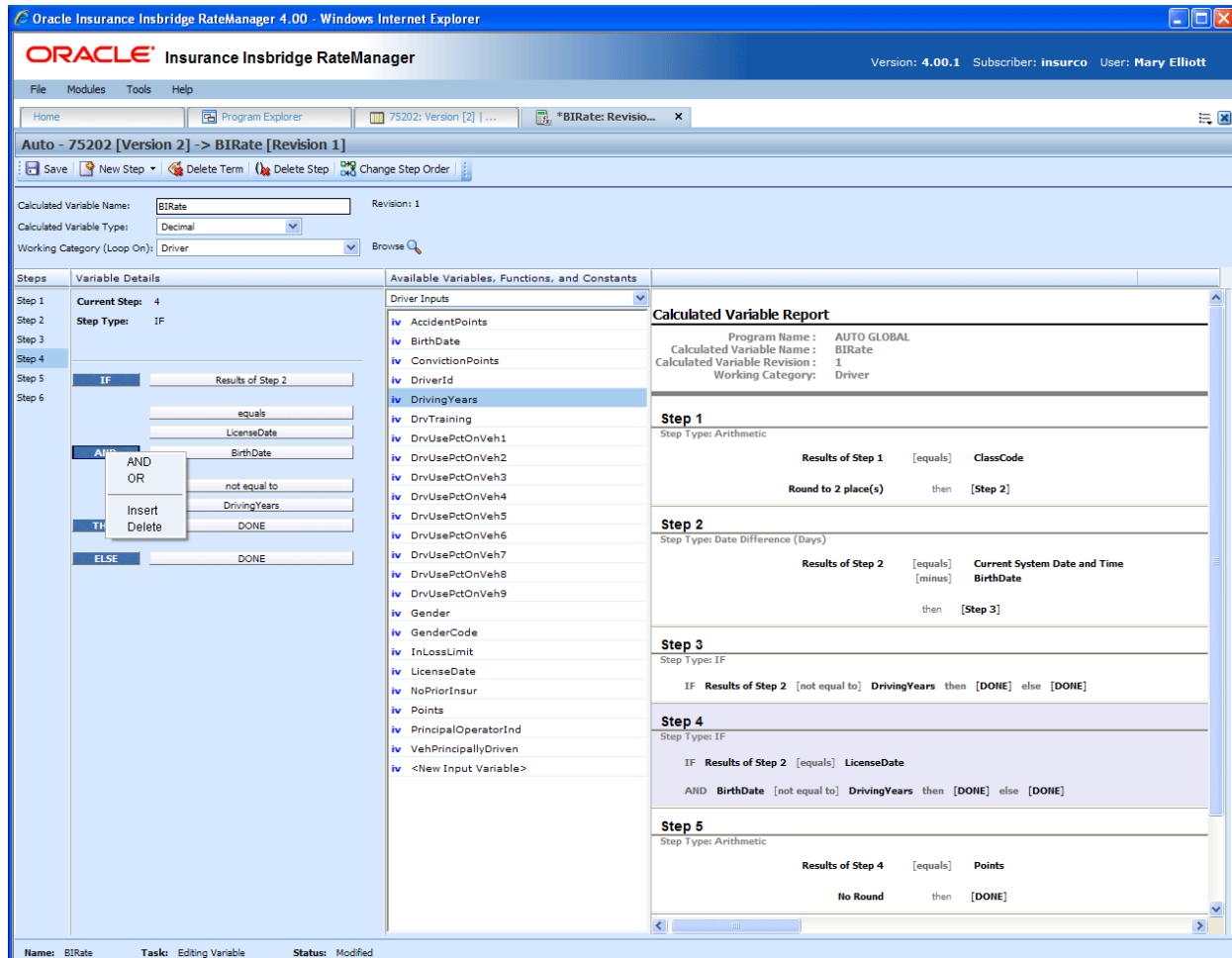
Figure 121 Editing a Multiple If Statement
