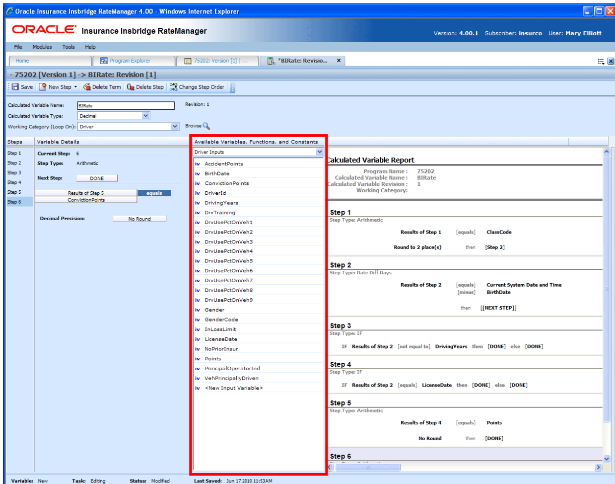
Figure 141 Available Variables, Functions and Constants Field
