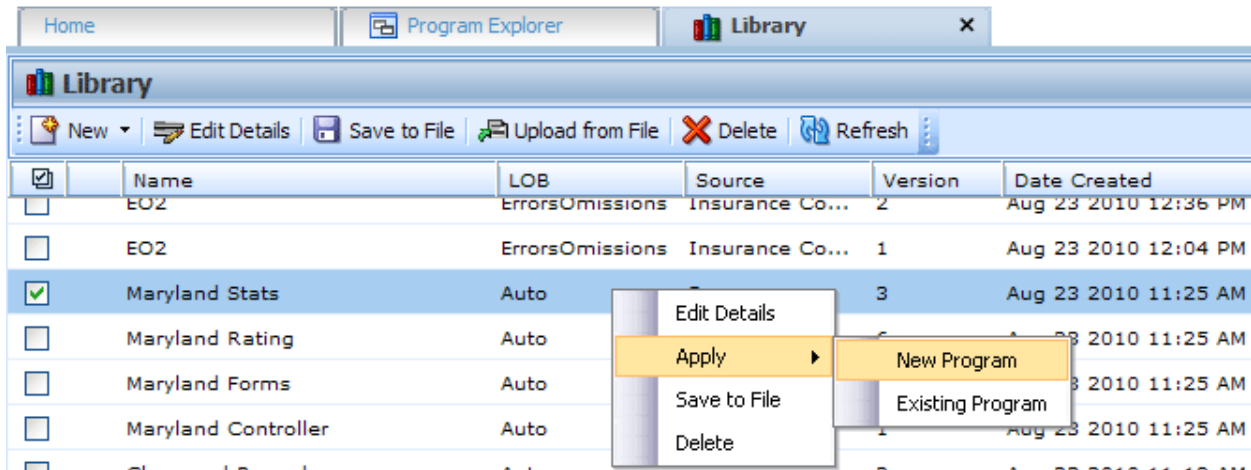
Figure 346 Applying a New Program
