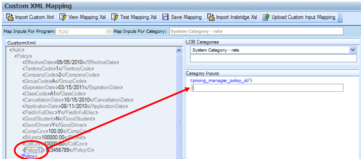
Figure 216 Mapping Custom XML
