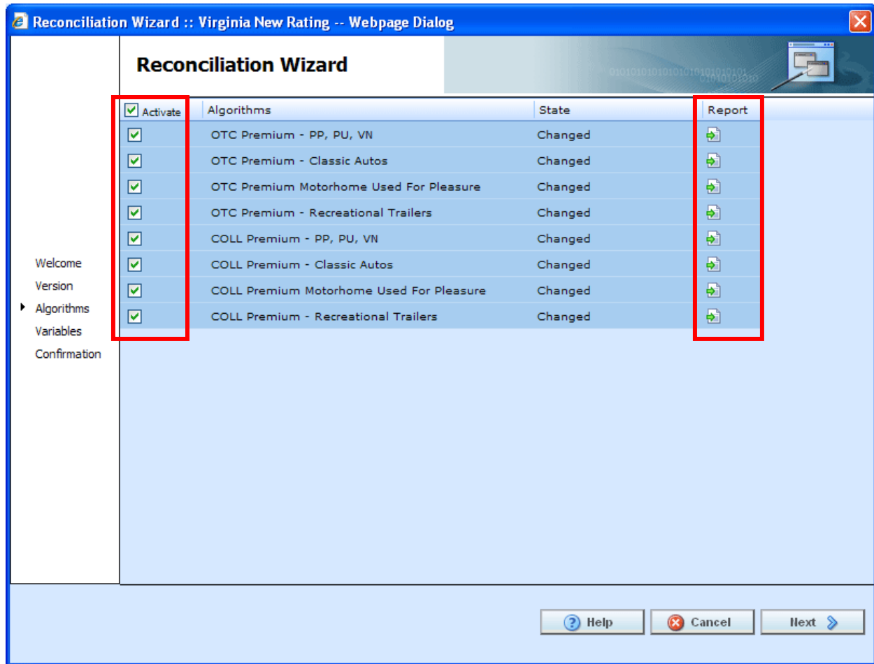
Figure 355 Reconciling Algorithms
