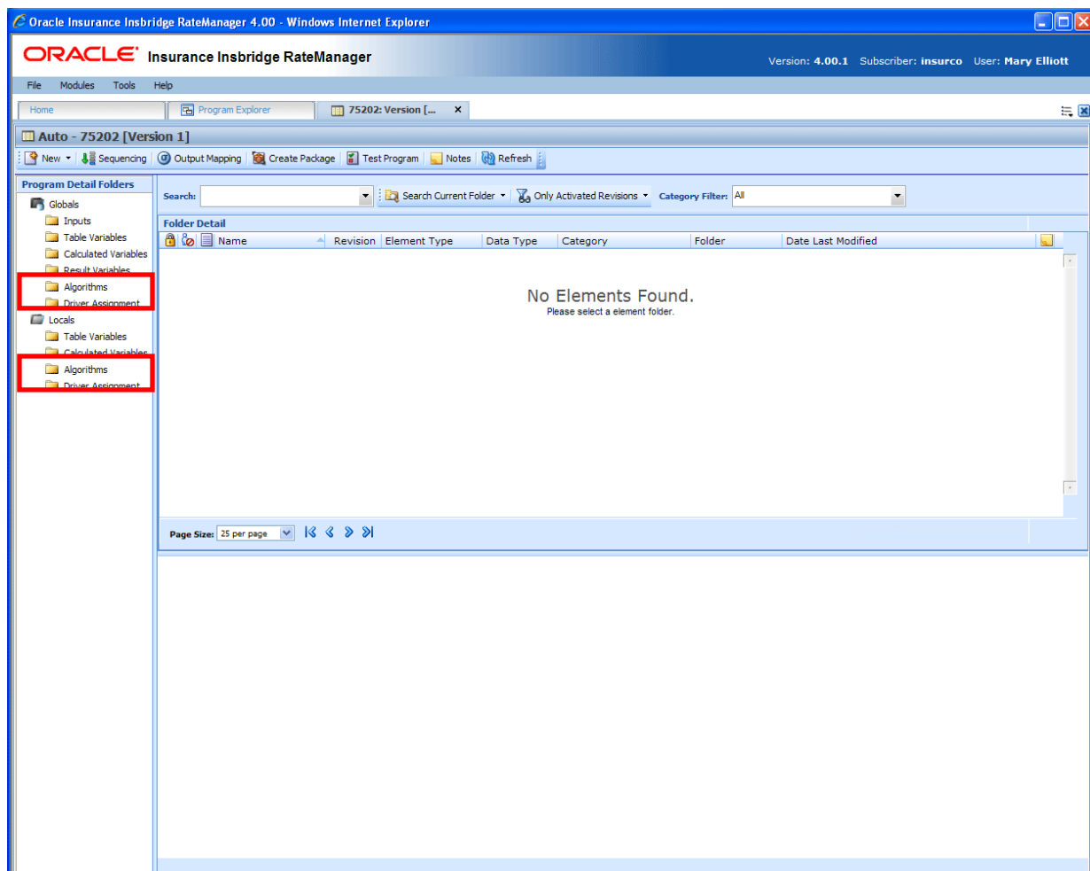
Figure 149 Algorithms Navigation
