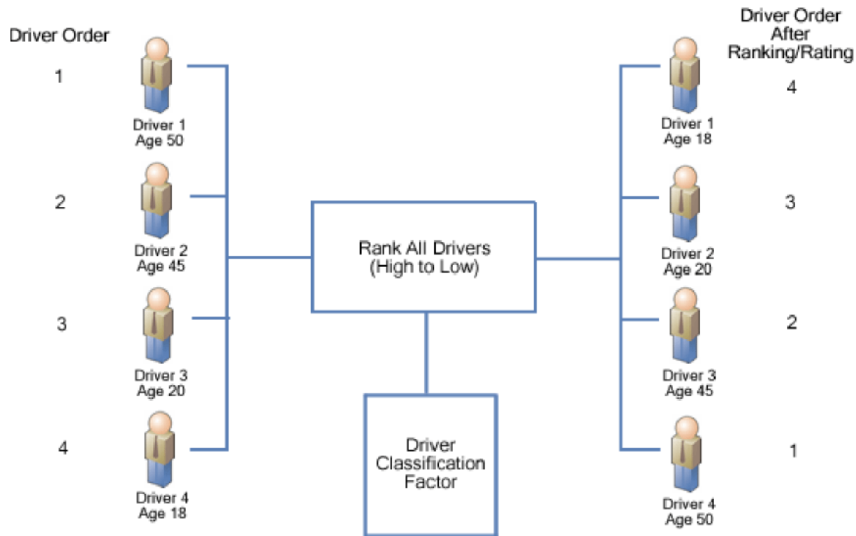
Figure 171 Ranking Functions
