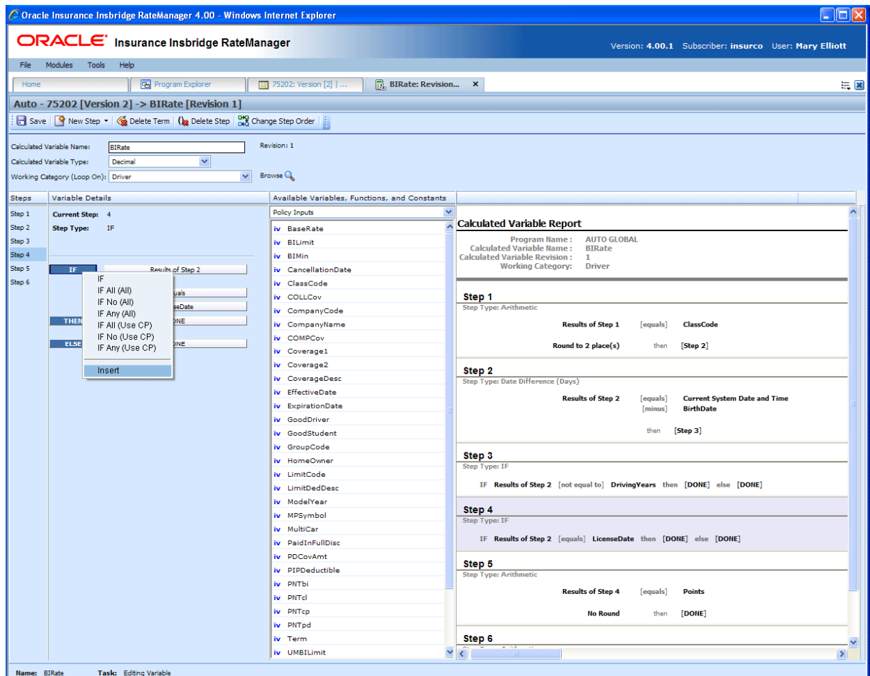
Figure 120 Creating a Multiple If Step
