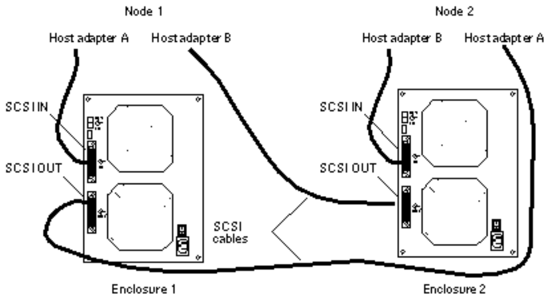
Figure 4-3 Example of a StorEdge MultiPack enclosure mirrored pair
