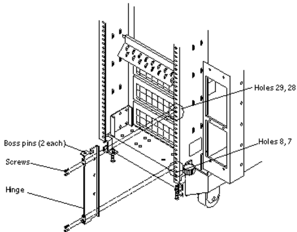
Figure 2-1 Installing the Terminal Concentrator Hinge
