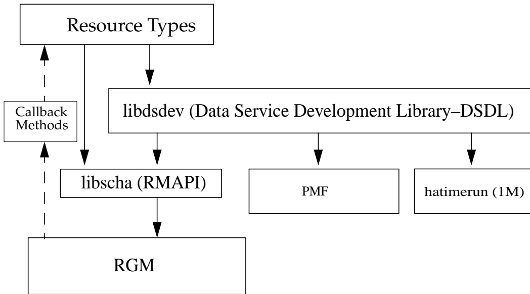
FIGURE 1-1 Programming Architecture
