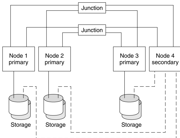
FIGURE 2-5 N+1 Topology
