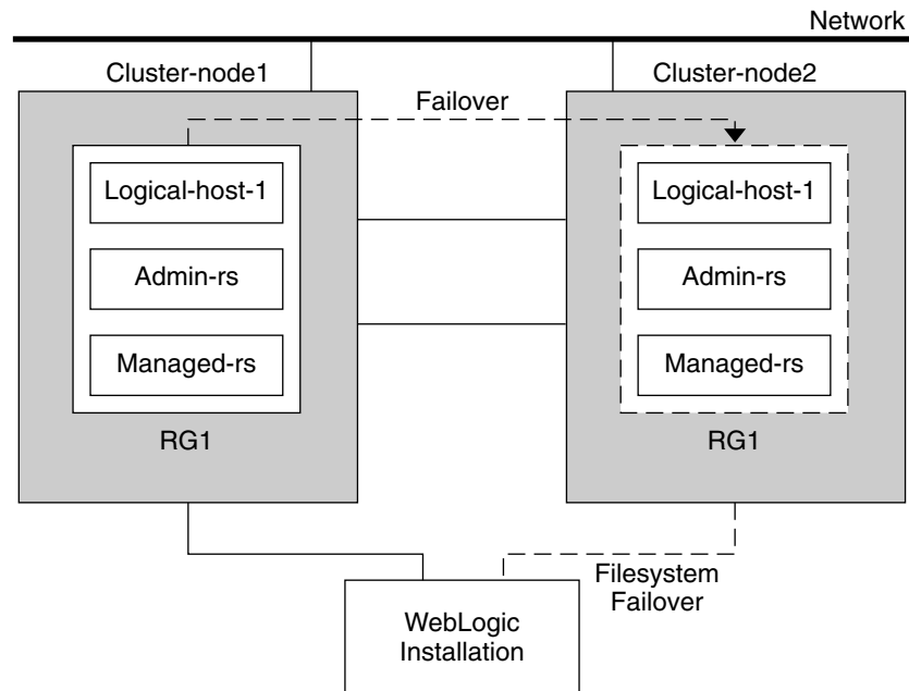
FIGURE 1-2 Sun Cluster HA for BEA WebLogic Server File System Failover Configuration
