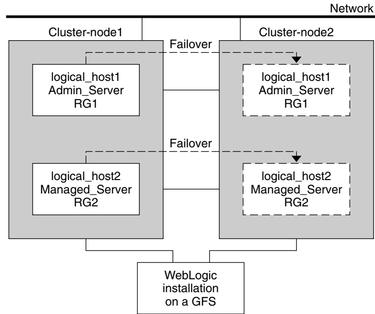
FIGURE 1-1 Sun Cluster HA for BEA WebLogic Server Simple Configuration
