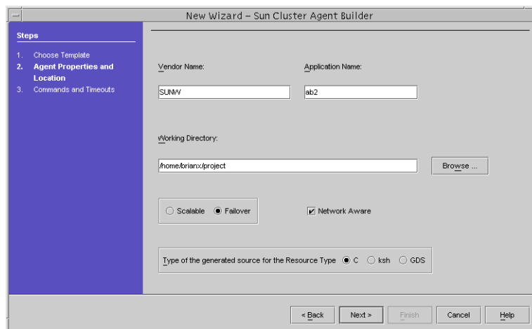
ABBILDUNG 9-5 Bildschirm "New Wizard - Sun Cluster Agent Builder" in Cluster Agent Module
