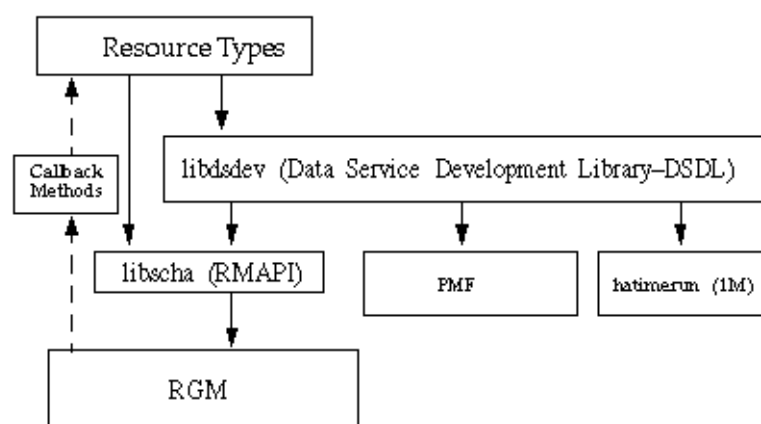
FIGURE 1-1 Architecture de programmation
