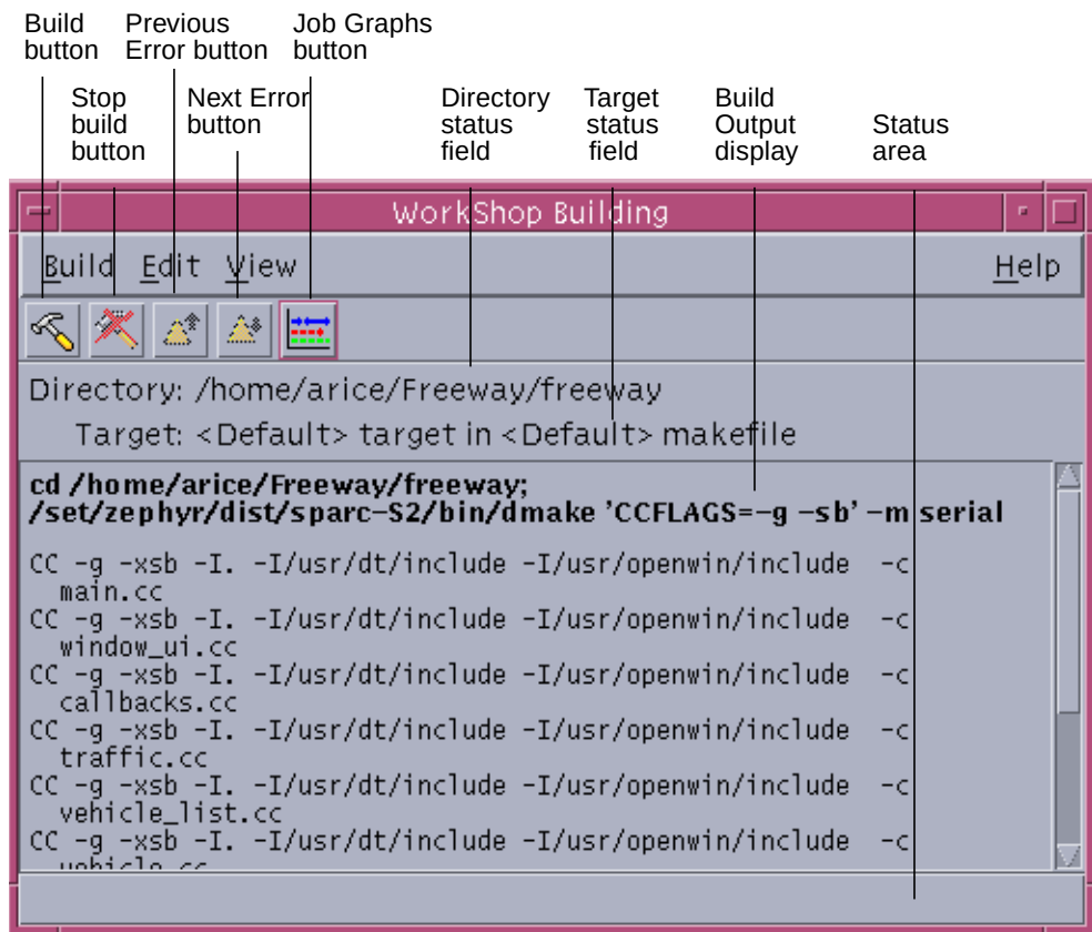
FIGURE 3-1 Building Window
