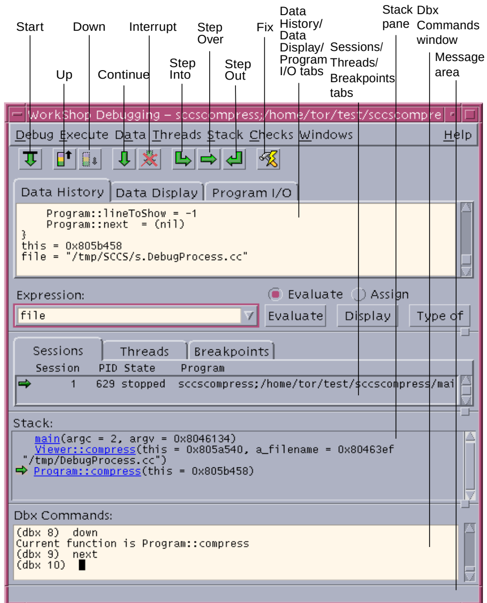
FIGURE 4-1 Debugging Window
