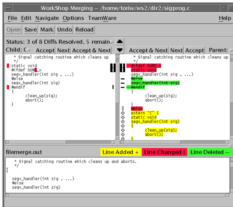
FIGURE 7-1 Merging Window
