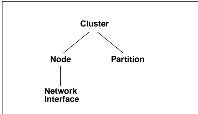
FIGURE 3-1 mpadmin Contexts
