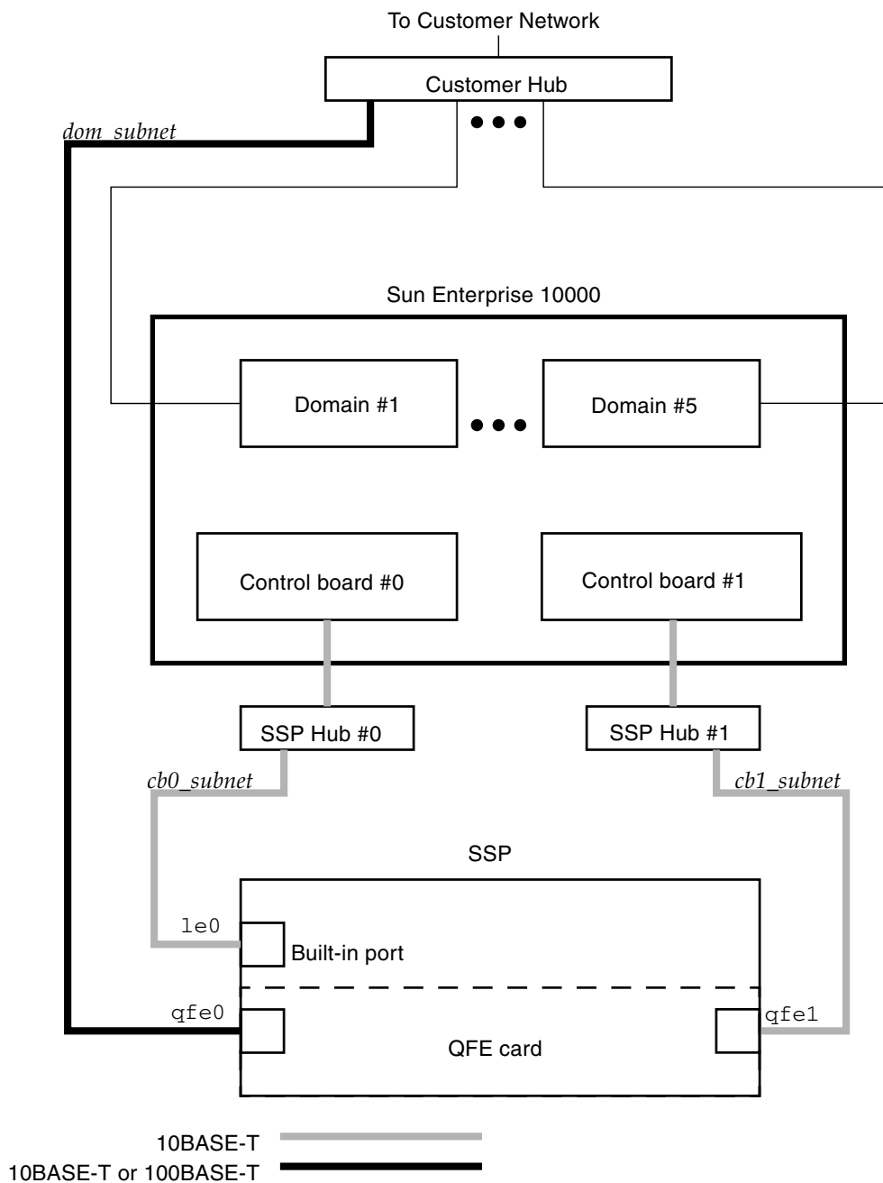
FIGURE 5-2 Network Configuration With Redundant Control Boards
