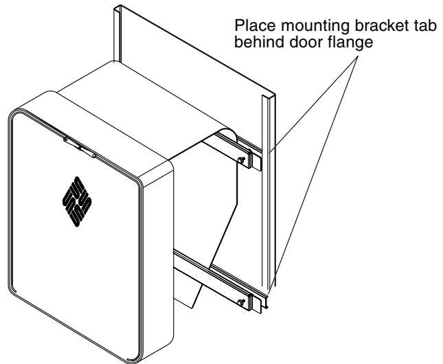
FIGURE 4-3 Mounting the Document Bag Assembly
