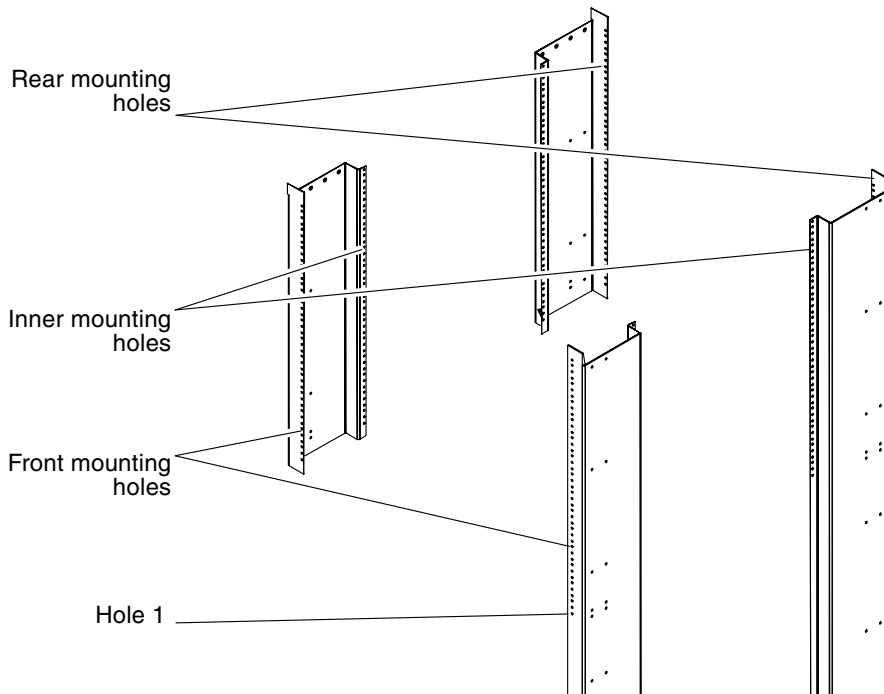
FIGURE 1-4 I/O Area Mounting Holes
