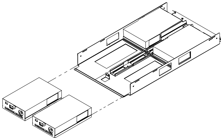
FIGURE 2-3 UniPack Disk Placement
