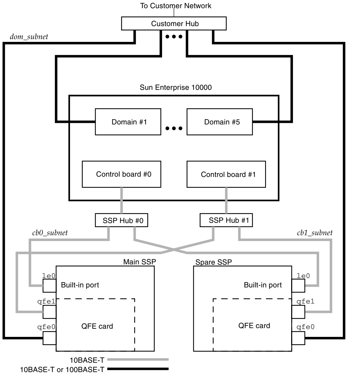
FIGURE 5-3 Network Configuration With Redundant Control Board and a Spare SSP
