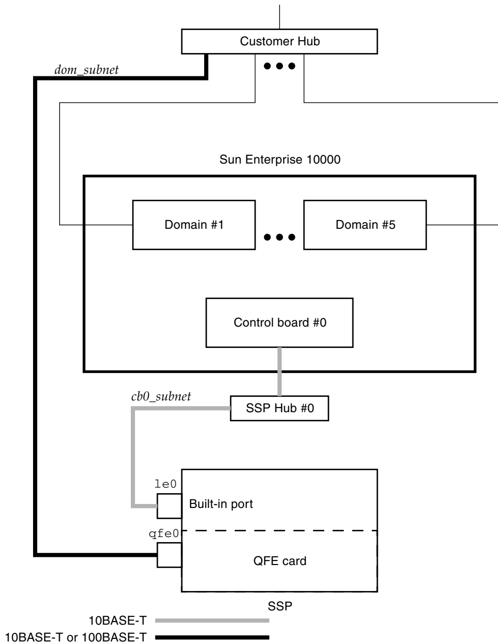
FIGURE 5-1 Network Configuration—Base Case
