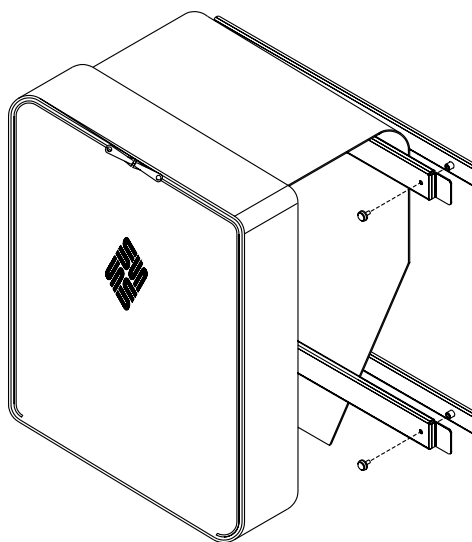
FIGURE 4-2 Assembling the Document Bag and Mounting Brackets
