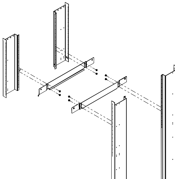
FIGURE 2-1 UniPack Rail Installation
