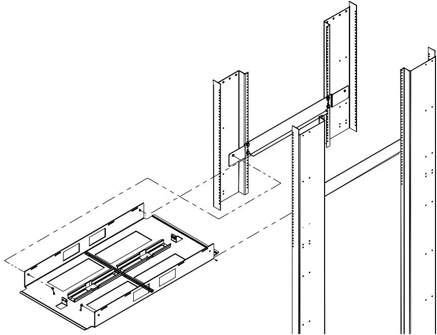
FIGURE 2-2 UniPack Tray Installation
