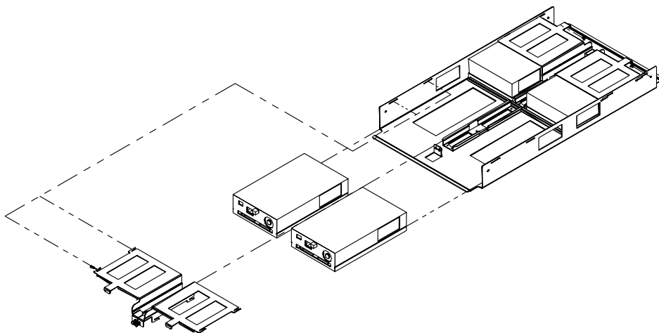
FIGURE 2-4 Securing the UniPack Disk
