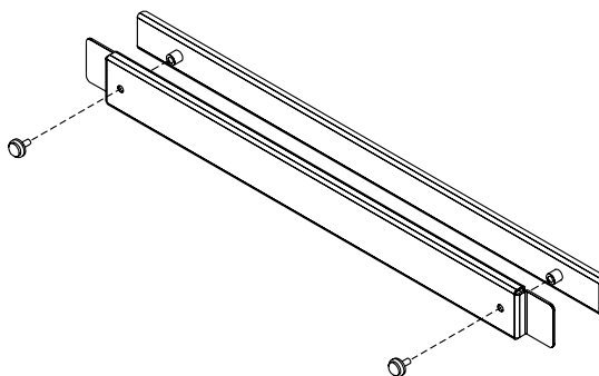
FIGURE 4-1 Document Bag Mounting Brackets
