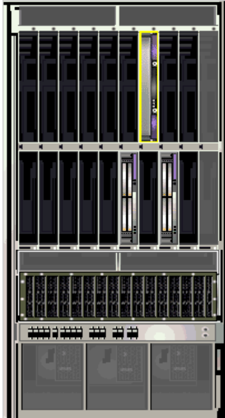
FIGURE 5-6 Sun Fire High-End Systems Domain Physical View—Front
