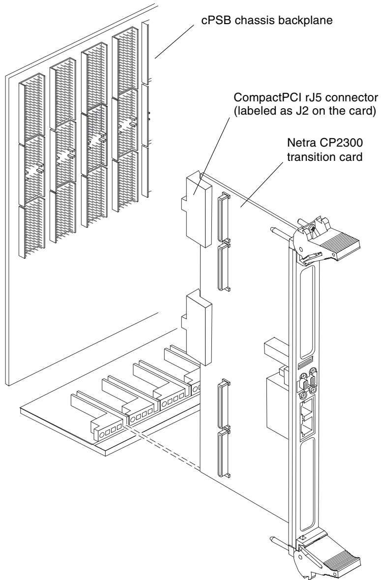
FIGURE 1-8 Align Transition Card During Installation in Backplane
