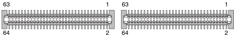
FIGURE A-7 PIM Connector Pins
