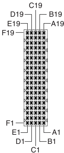
FIGURE A-9 CompactPCI rJ3 Connector (J1) Pins
