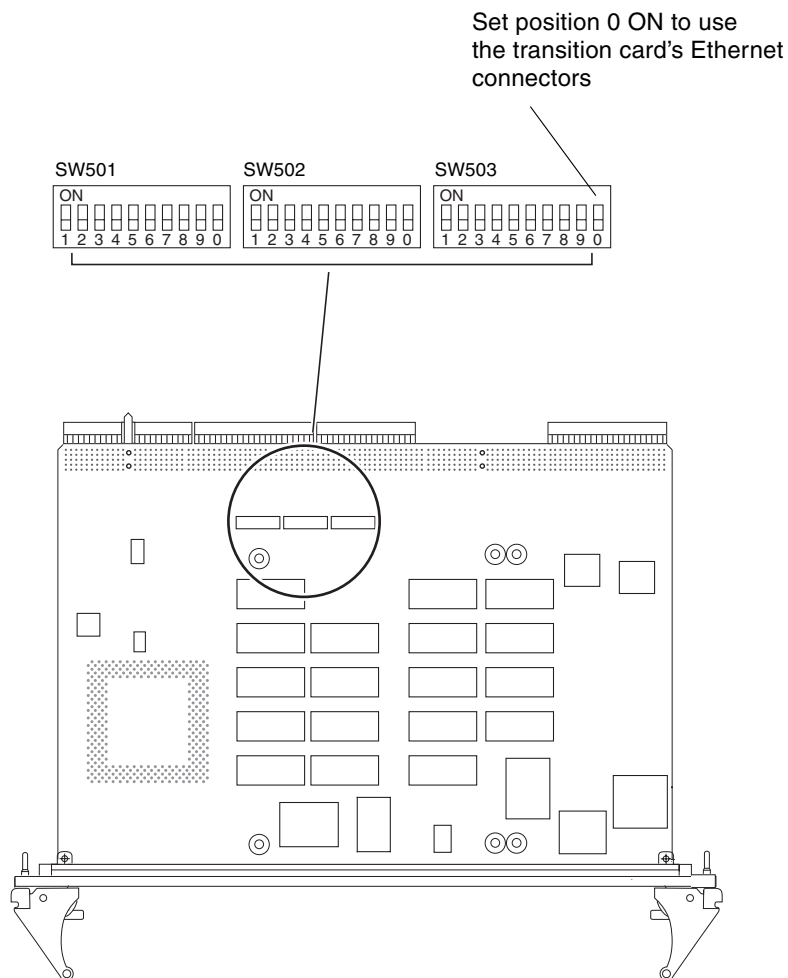
FIGURE A-4 Setting the SW503 DIP Switch on the Netra CP2300 cPSB Board
