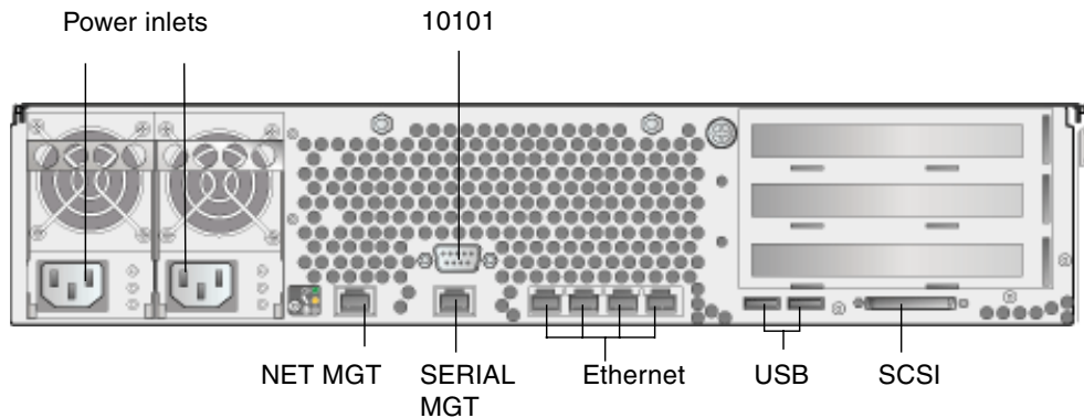
FIGURE 2 Sun Fire V240 Server Back Panel
