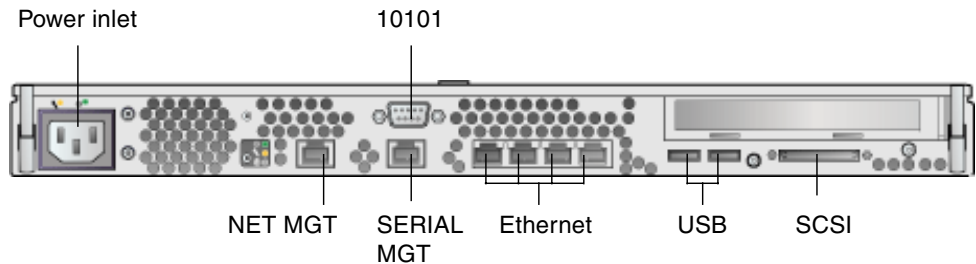
FIGURE 1 Sun Fire V210 Server Back Panel
