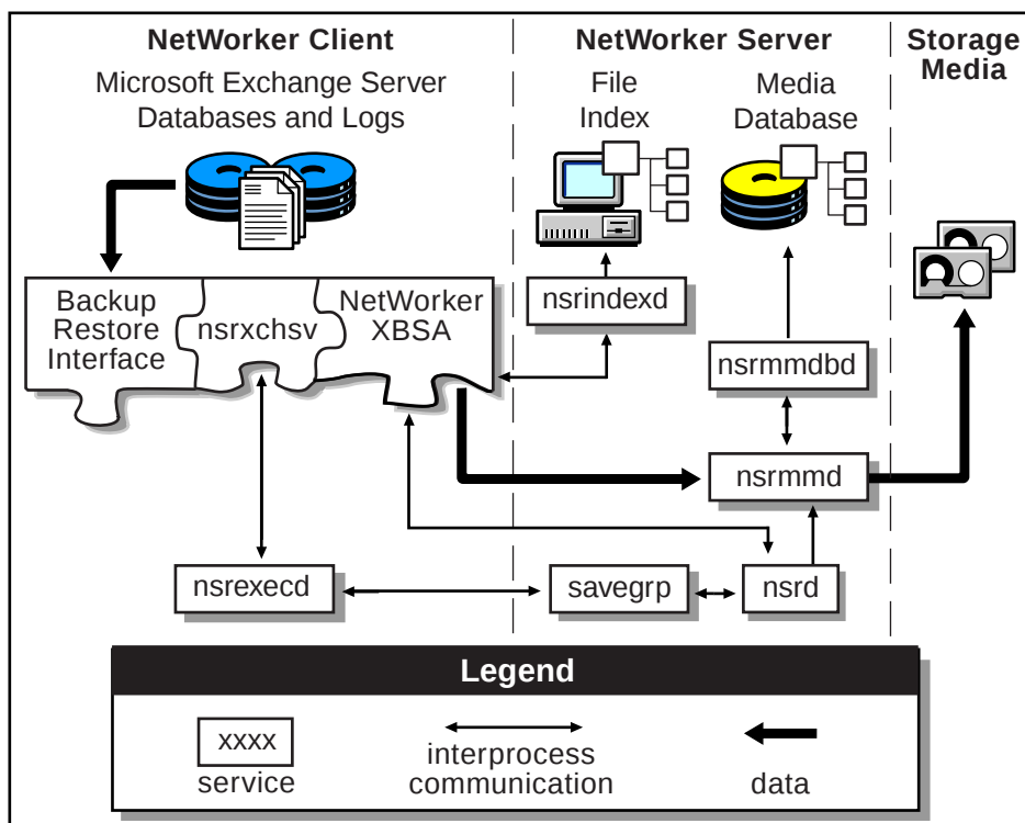
Figure 1. NetWorker Client-Server Interaction During a Backup Initiated by NetWorker Module
