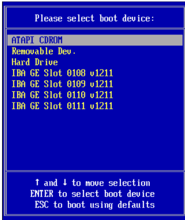
FIGURE 7-2 Menu Boot Device
