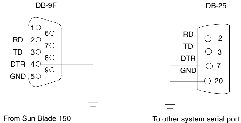
FIGURE 7 Crossover Serial Cable Wiring for Tip Connections, 9-pin to 25-pin
