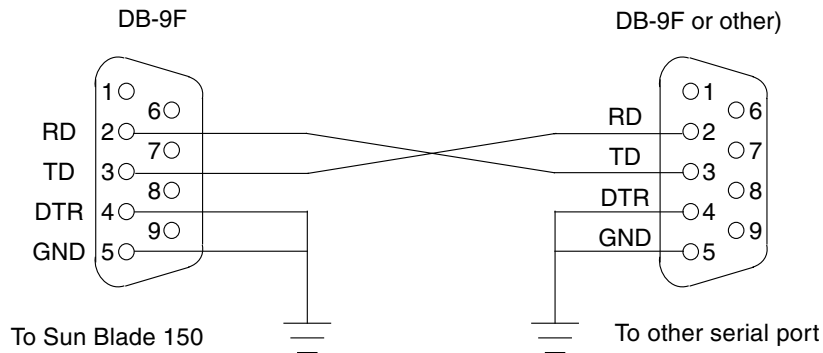
FIGURE 6 Crossover Serial Cable Wiring for Tip Connections, 9-pin to 9-pin
