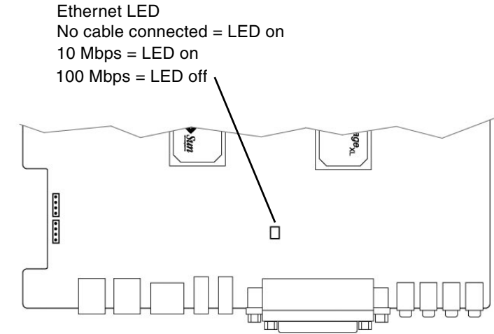
FIGURE 5 Ethernet LED on Motherboard
