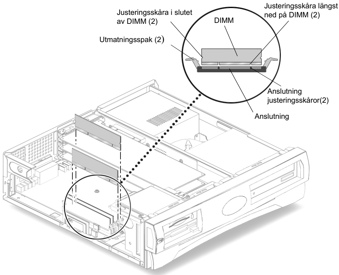
FIGUR 4-7 Installera DIMM:ar
