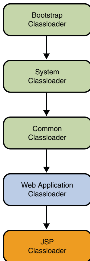
FIGURE 9-1 Classloader Runtime Hierarchy
