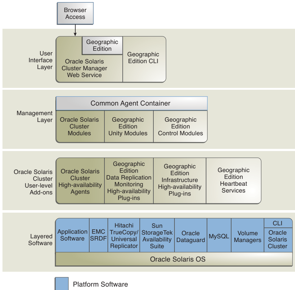
FIGURE 3-1 Overview of Geographic Edition Software Architecture
