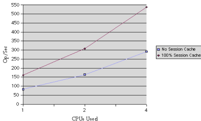
Figure 7-8 SSL Test: C CGI
