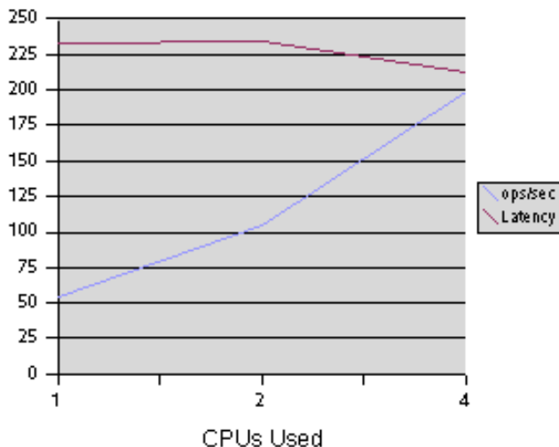
Figure 7-11 PHP Scalability Test: FastCGI
